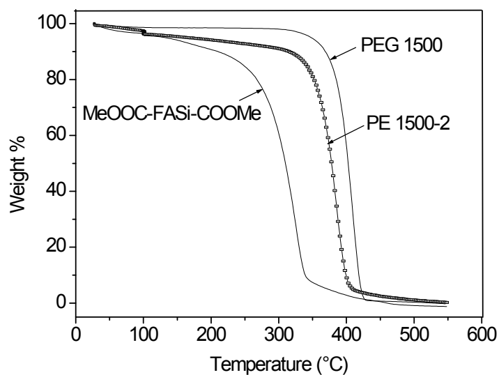
Thermal decomposition profiles of PE 1500-2, PEG 1500 and MeOOC-FASi-COOMe.
