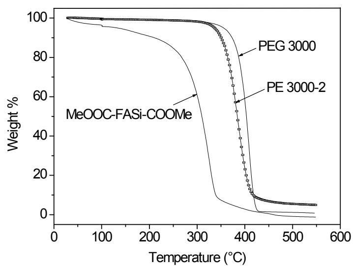
Thermal decomposition profiles of PE 3000-2, PEG 3000 and MeOOC-FASi-COOMe.
