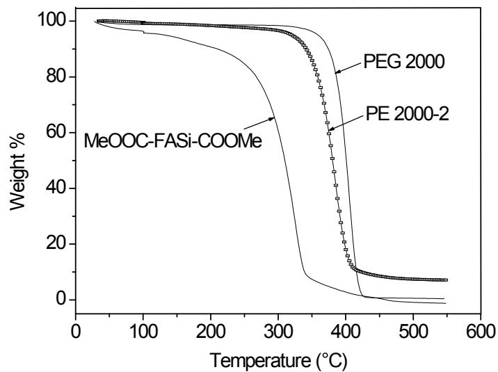
Thermal decomposition profiles of PE 2000-2, PEG 2000 and MeOOC-FASi-COOMe.
