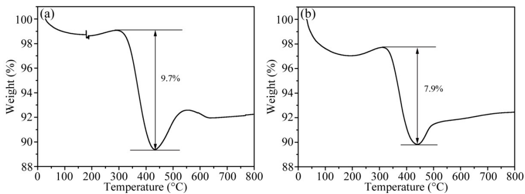
Fig. A3 TG curves of S2 (a) and S3 (b).
