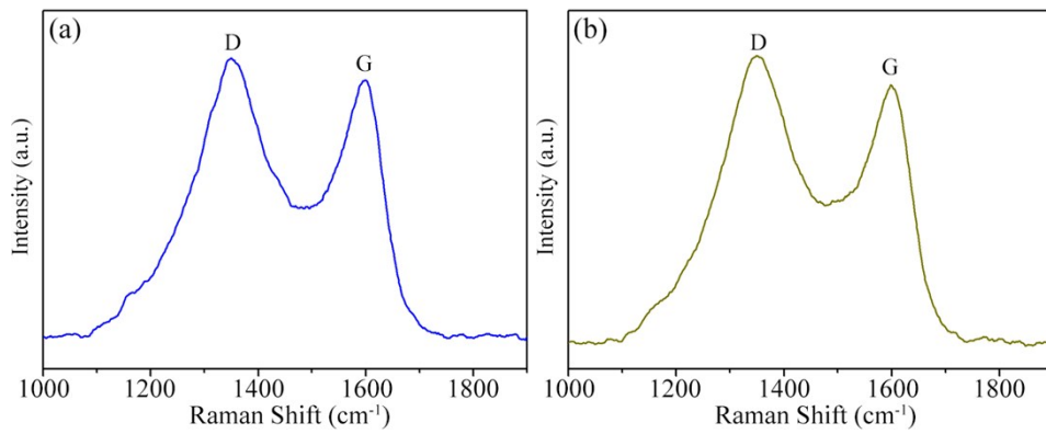
Fig. A2 Raman spectra of S2 (a) and S3 (b).
