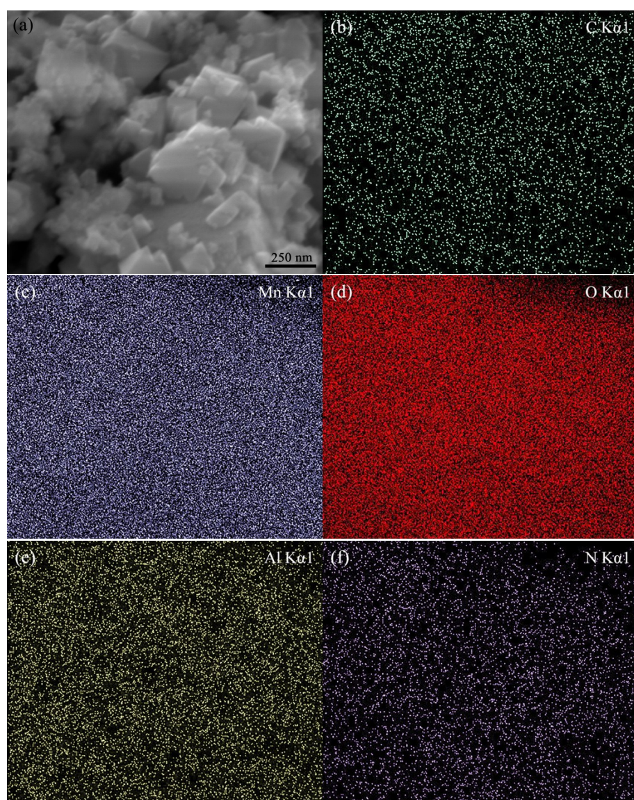
Fig. A1 FESEM image and the corresponding elemental mappings of S3.
