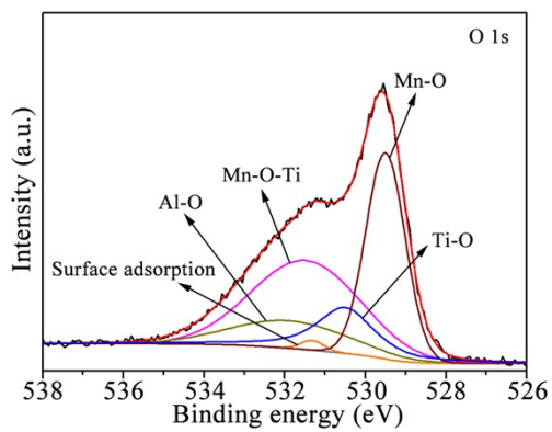
Fig. A4 XPS spectrum of O1s for S1.
