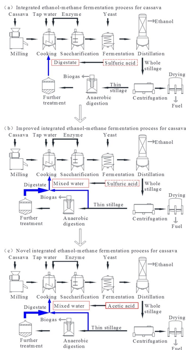
Supplementary fig. 1: Process diagram of the integrated process (a), improved integrated process (b) and novel integrated process (c) for cassava ethanol production.
