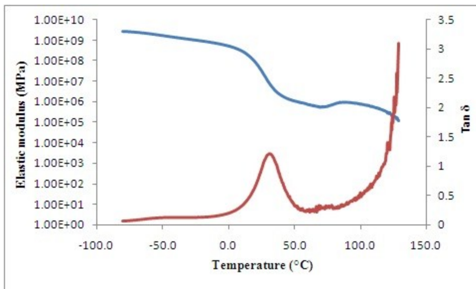
Fig. S1. Temperature dependence of the storage modulus and \tan \delta for PVB.
