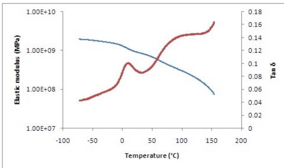
Fig. S2. Temperature dependence of the storage modulus and \tan \delta for PP.
