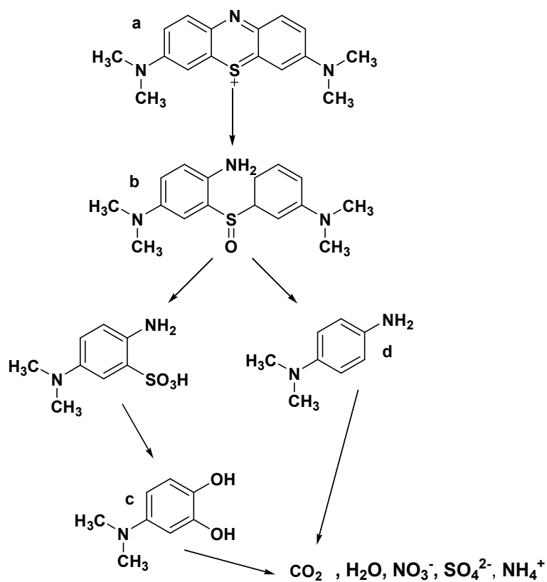
Scheme S1.
