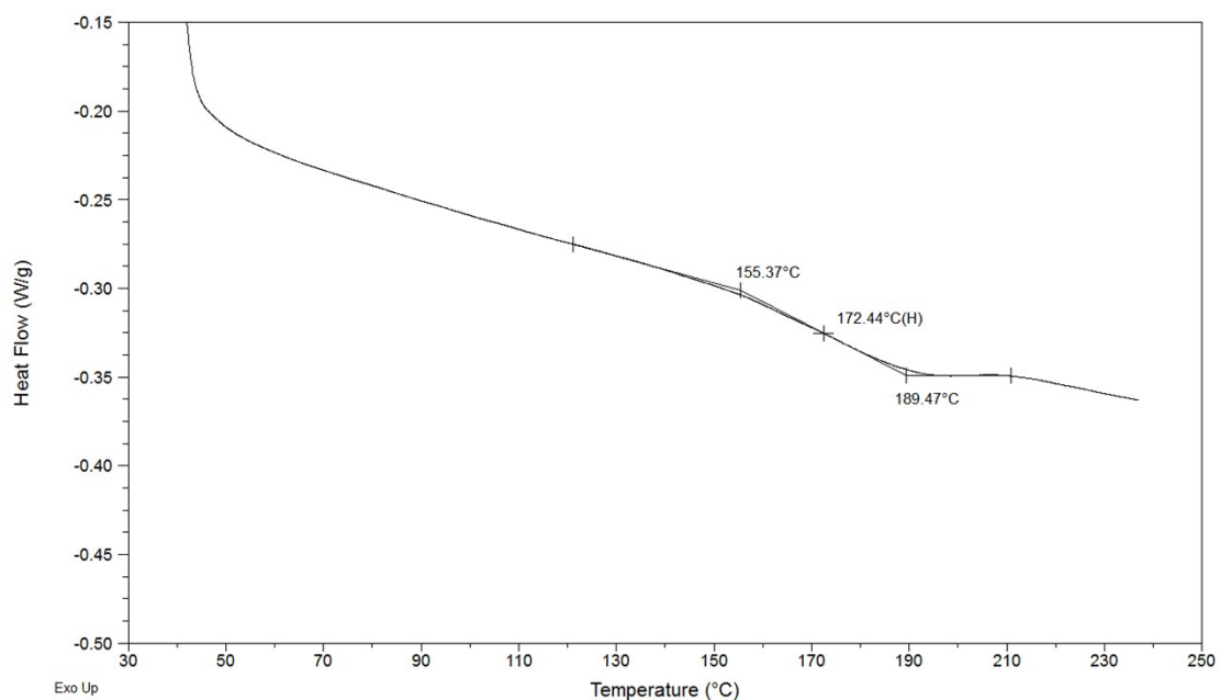
Fig. S2 DSC thermogram of compound 1 .
