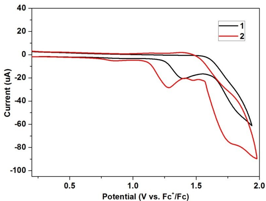
Fig. S1 Cyclic voltammograms of compounds 1 and 2 in CH 2 Cl 2 solutions (10 -3 M). Potentials were recorded versus Fc + /Fc.
