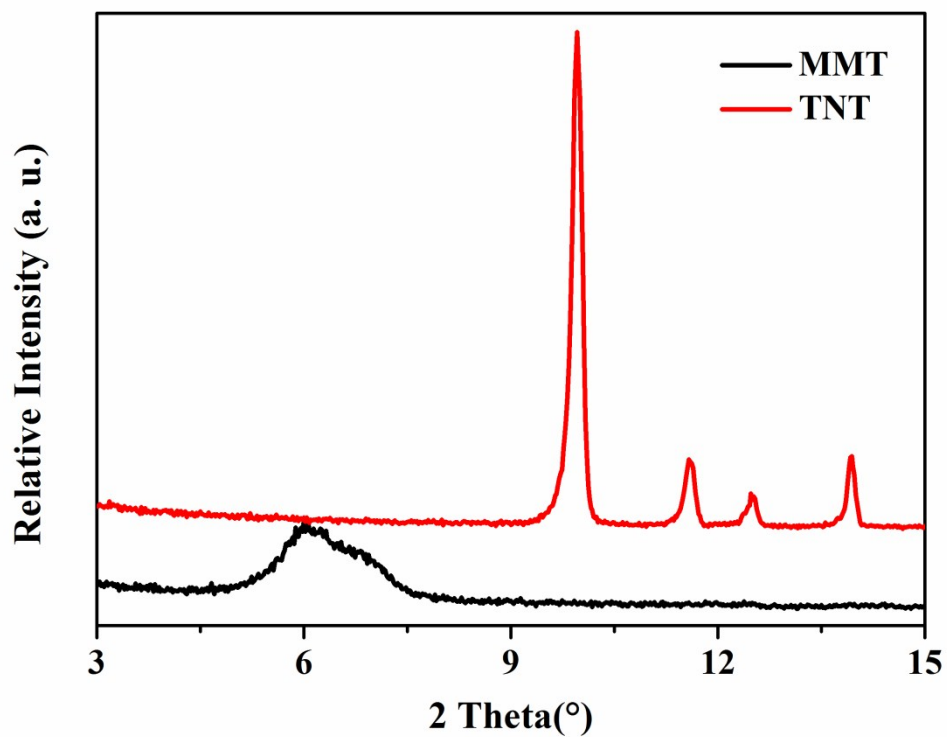
Figure S1. XRD patterns of MMT and TNT.
