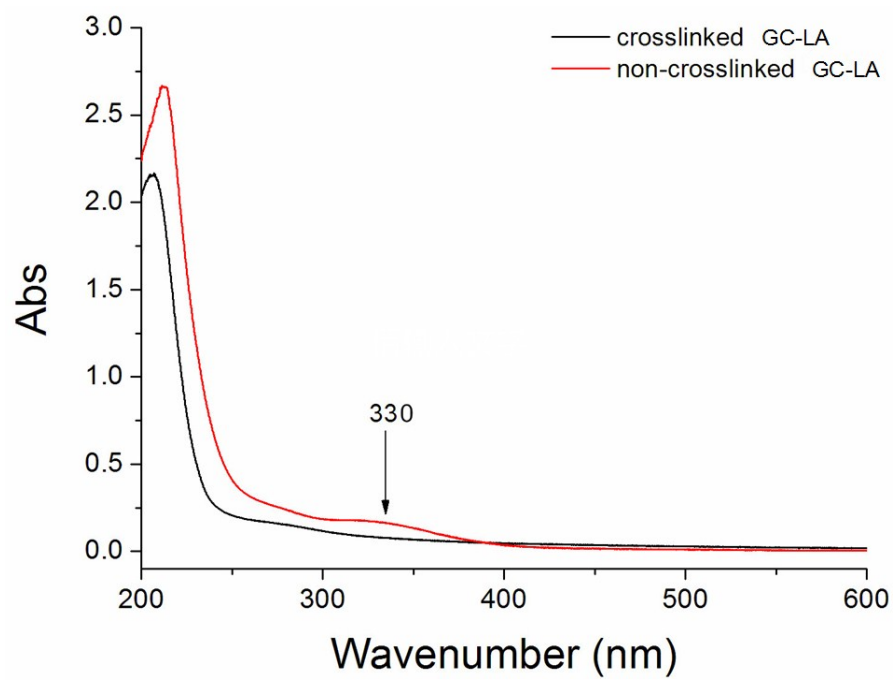
Fig. S2 UV-vis absorption spectra of GC-LA and GC-LA/cc micelles.
