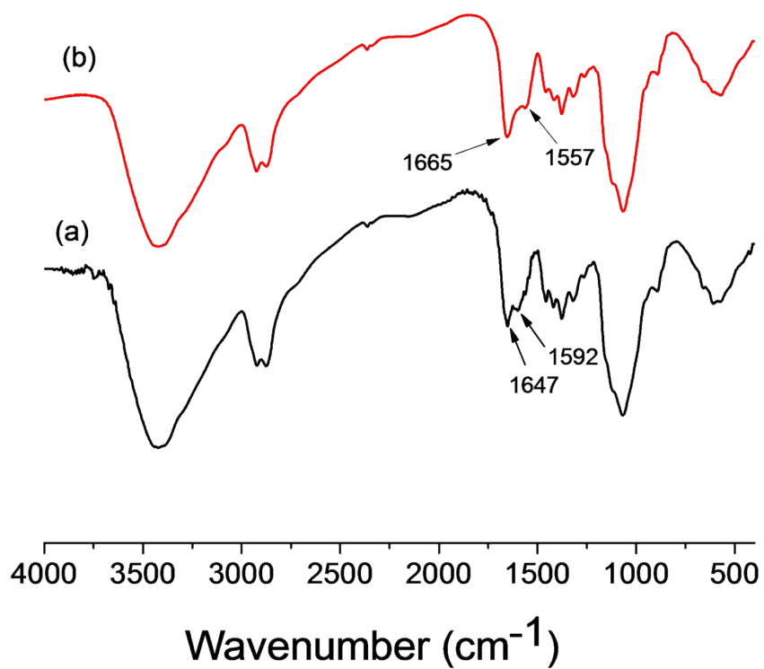
Fig. S1 Fourier-transform infrared spectra of (a) glycol chitosan and (b) GC-LA.
