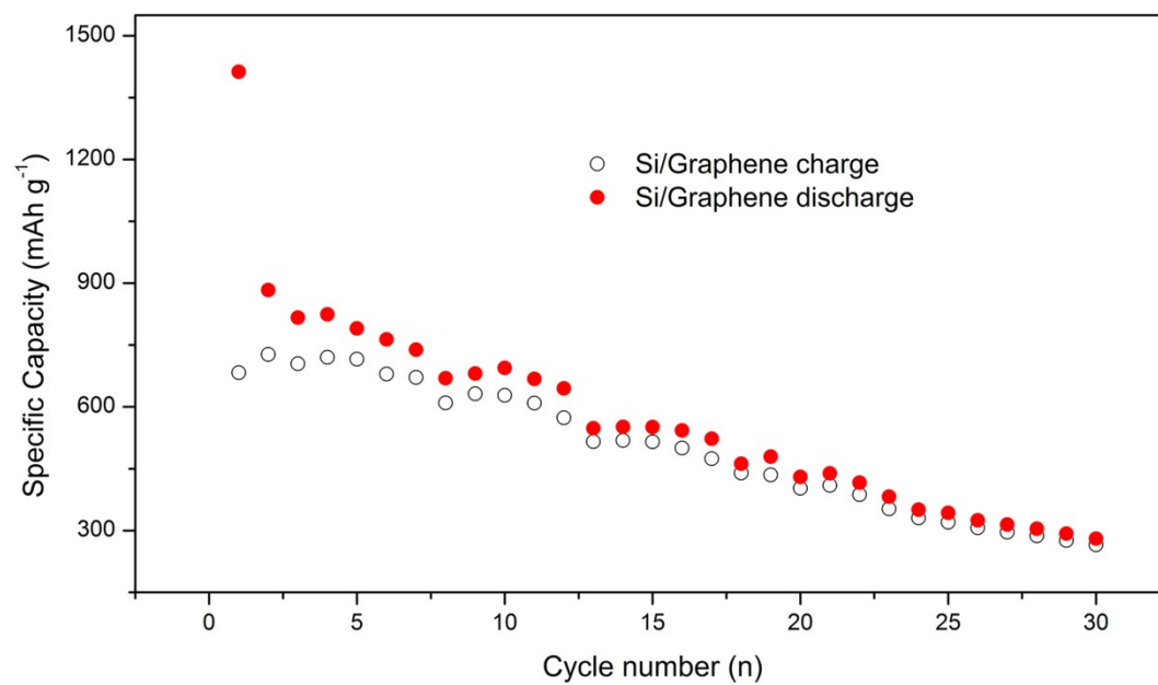
Figure.S1 Cyclability data of physical mixture of Si/Graphene
