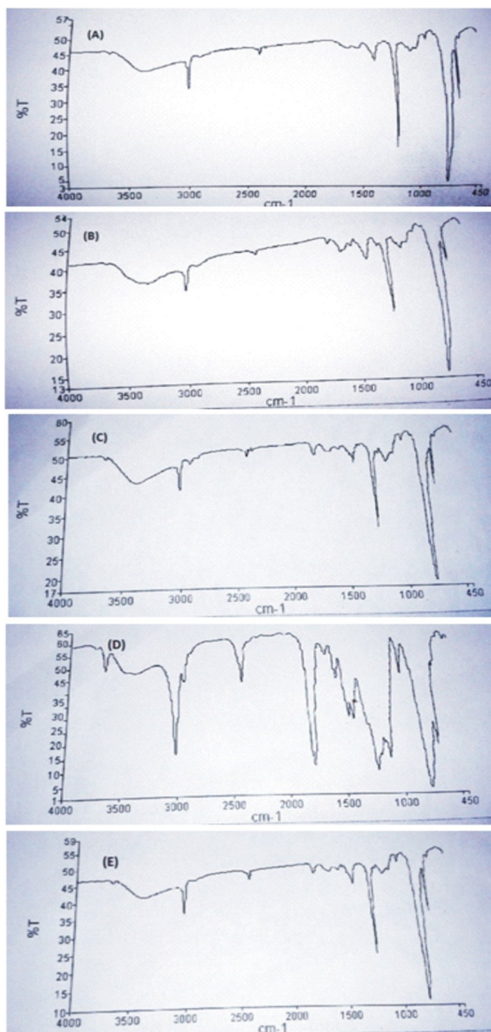
Supplementary figure 1. FTIR Spectra of (A) AmB, (B) Dox, (C) Formulation, (D) Physical mixture, (E) PLGA.
