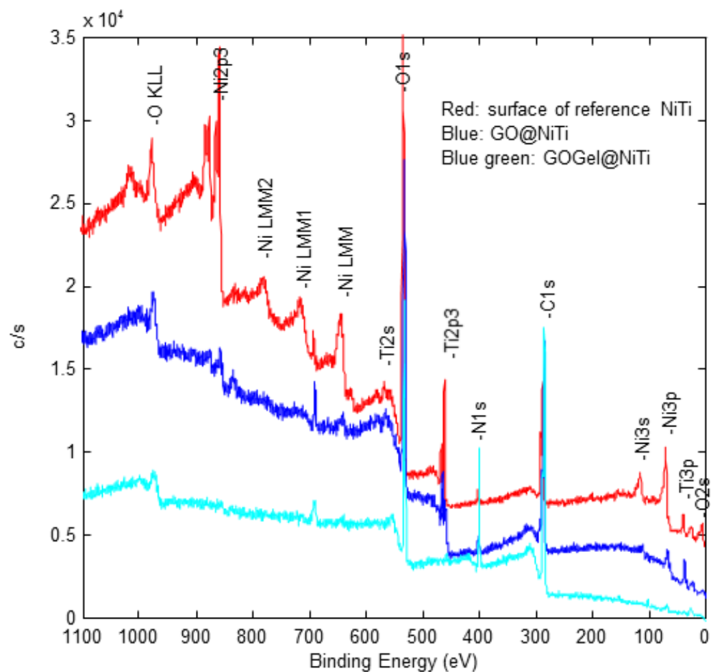
Fig. S1 Typical XPS survey spectra of GO@NiTi, GOGel@NiTi and NiTi surfaces.
