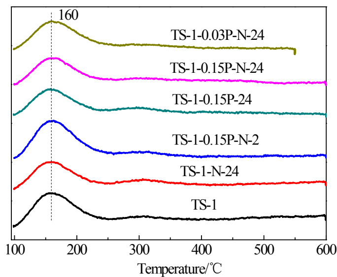
Figure 2 The NH 3 -TPD curves of TS-1 and the modified samples
