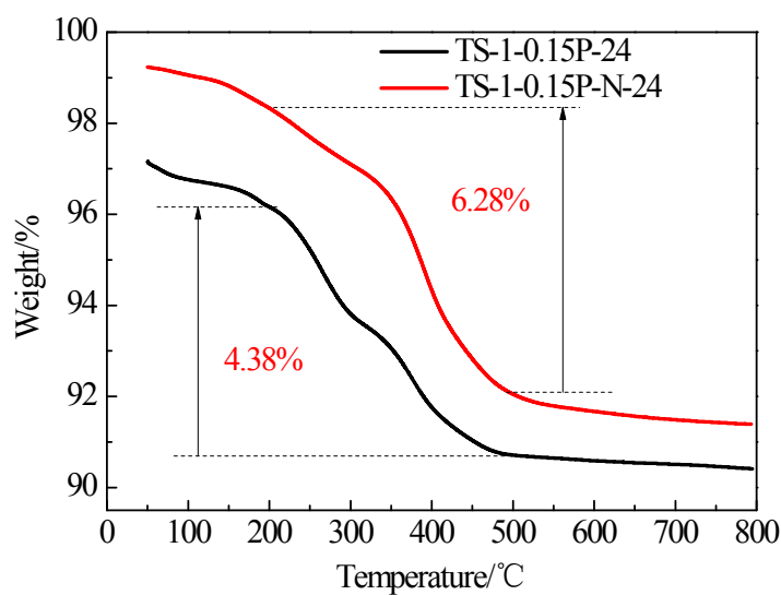
Figure 1 The TGA curves of uncalcined TS-1-0.15P-24 and TS-1-0.15P-N-24
