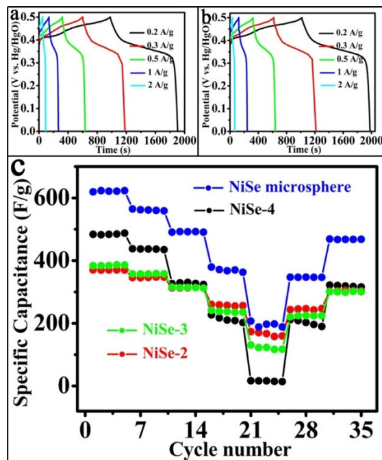
Figure S2 (a and b) The galvanostatic charge-discharge curves of NiSe-2 and NiSe-3 at various current densities respectively; (c) Discharge specific capacitance curves of NiSe-2, NiSe-3, NiSe-4 and NiSe microspheres
