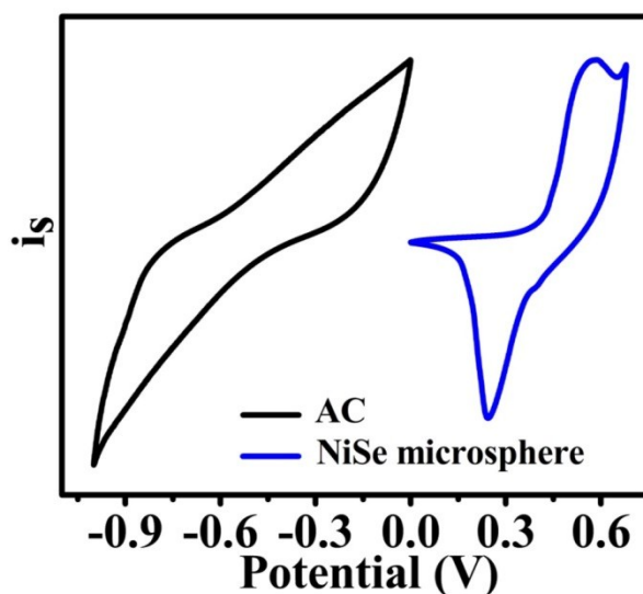
Figure S1 Normalized CV curves of AC and NiSe microspheres at the scan rate of 5 mV s -1
