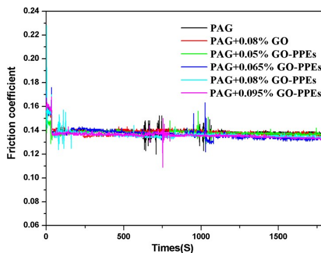
Fig. S1 Friction coefficient of the discs lubricated by PAG, 0.08% GO and PAG with different concentrations of GO-PPEs composites at 25 °C (SRV load, 25 N; stroke, 1 mm; frequency, 25 Hz).
