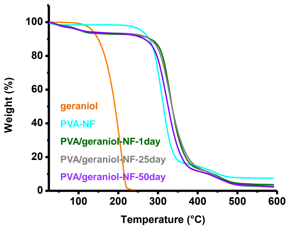
Figure S2. TGA of geraniol, PVA-NF, PVA/geraniol-NF-1day, PVA/geraniol-NF-25day, and PVA/geraniol-NF-50day.
