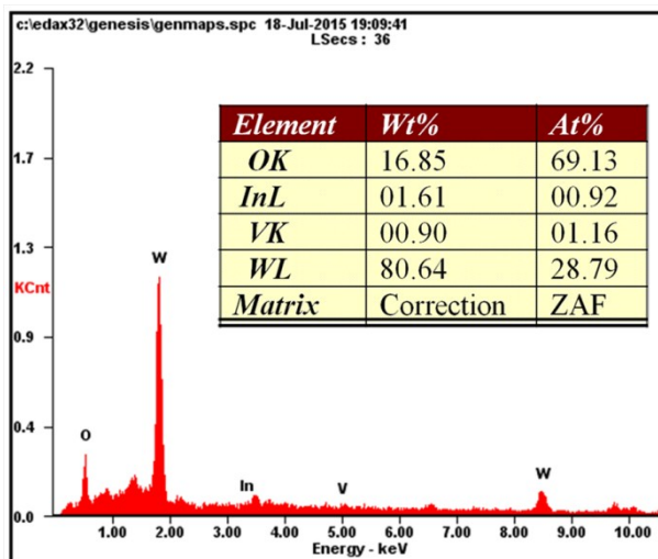
Fig. S1 The EDS spectra of InVO 4 /WO 3 films
