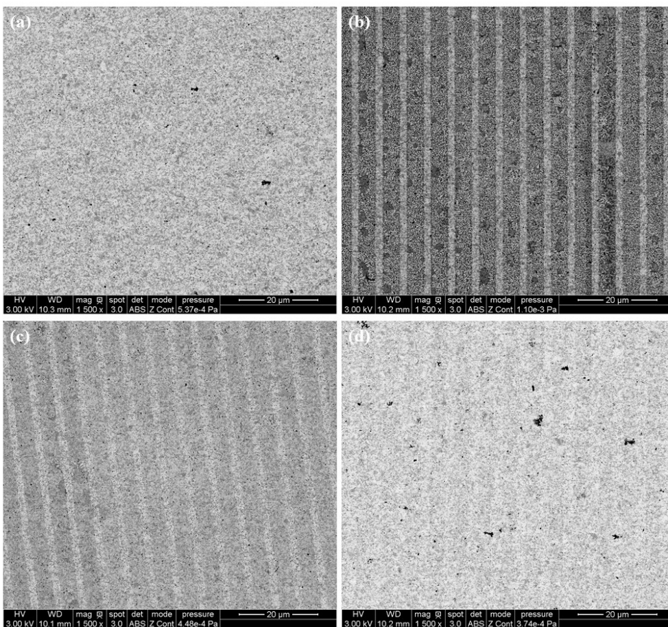
Figure 12 Backscattered electron images of magnetite co-precipitated on ODT-PEG patterned surfaces treated with (a) buffer, (b) Mms6, (c) m2Mms6 and (d) BSA.
