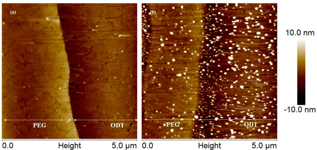
Figure 11 Tapping mode AFM of ODT-PEG patterned surface treated with buffer (a) and BSA (b)
