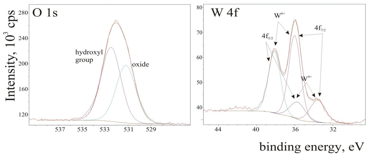
Figure S1. Detailed XPS scans of core O 1s and W 4f levels of the WO_{3-x} nanocrystals on a Si wafer.
