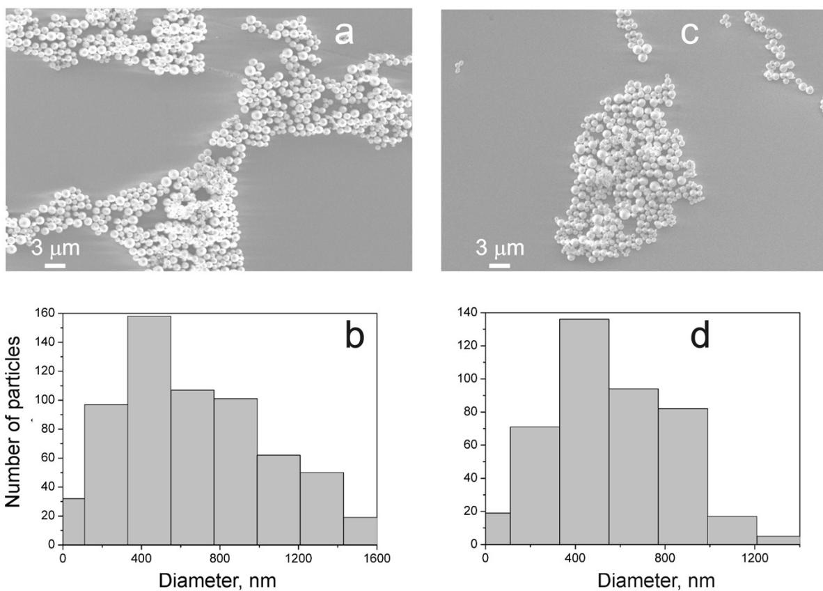
Figure S2. Representative SEM images and corresponding size histograms of the \text{WO}_{3-x} nanocrystals on a Si wafer deposited from water (a,b) and acidic solution (c,d) respectively.
