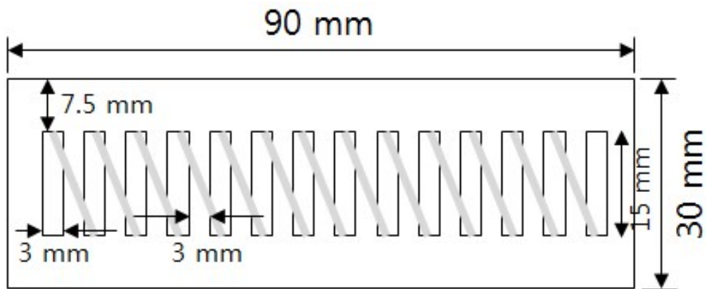
Fig. S1 Photograph and schematic of the CNT/PEDOT:PSS OTEG.
