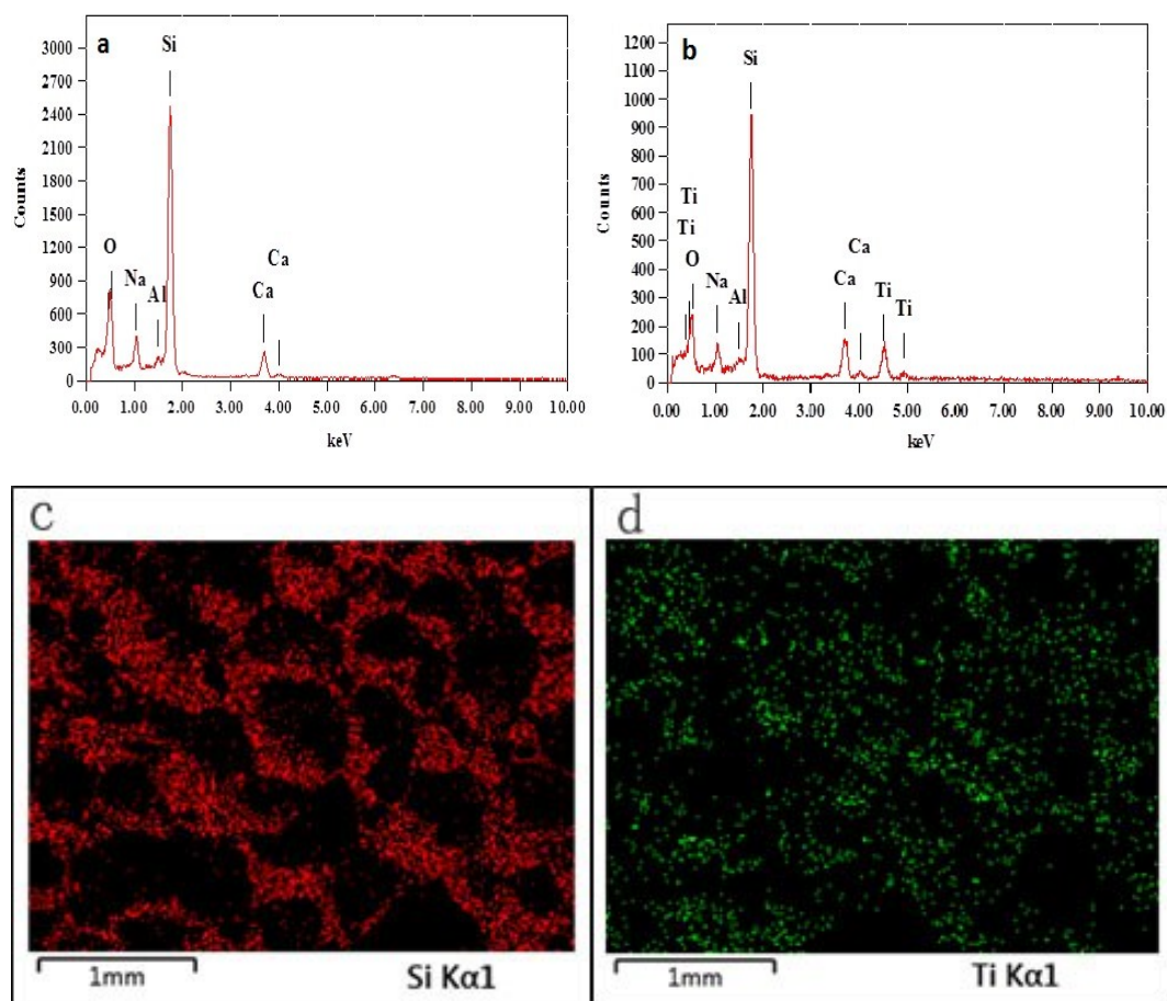
Figure S2 EDX patterns of the (a) FG and (b) p-TiO 2 /FG, element mapping of (c) Si and (d) Ti on p-TiO 2 /FG.
