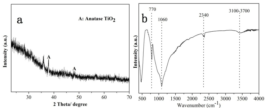
Figure S4 (a) XRD patterns and (b) FTIR spectra of the p-TiO 2 /FG photocatalyst after the wastewater treatment process
