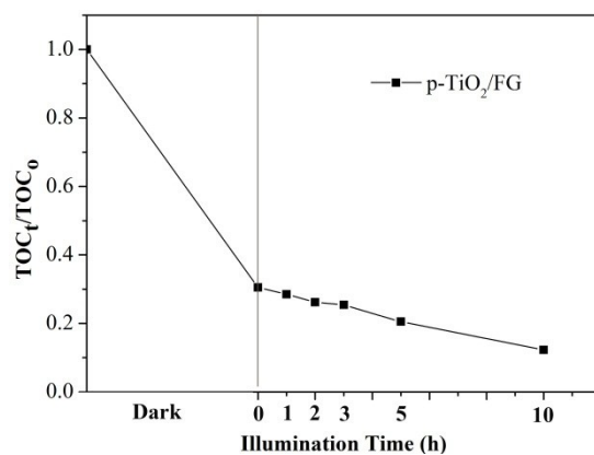
Figure S3 TOC removal efficiency of the MB aqueous solution using p-TiO 2 /FG as photocatalyst with UV light illumination
