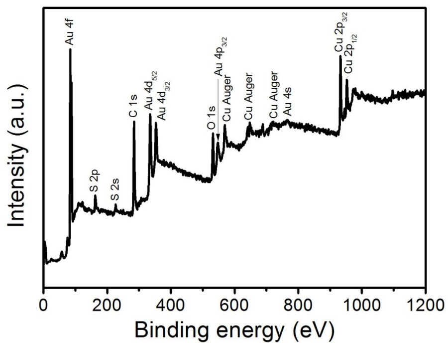
Figure S1. XPS full spectrum of the as-prepared rGO/CuS/Au composite nanosheets.
