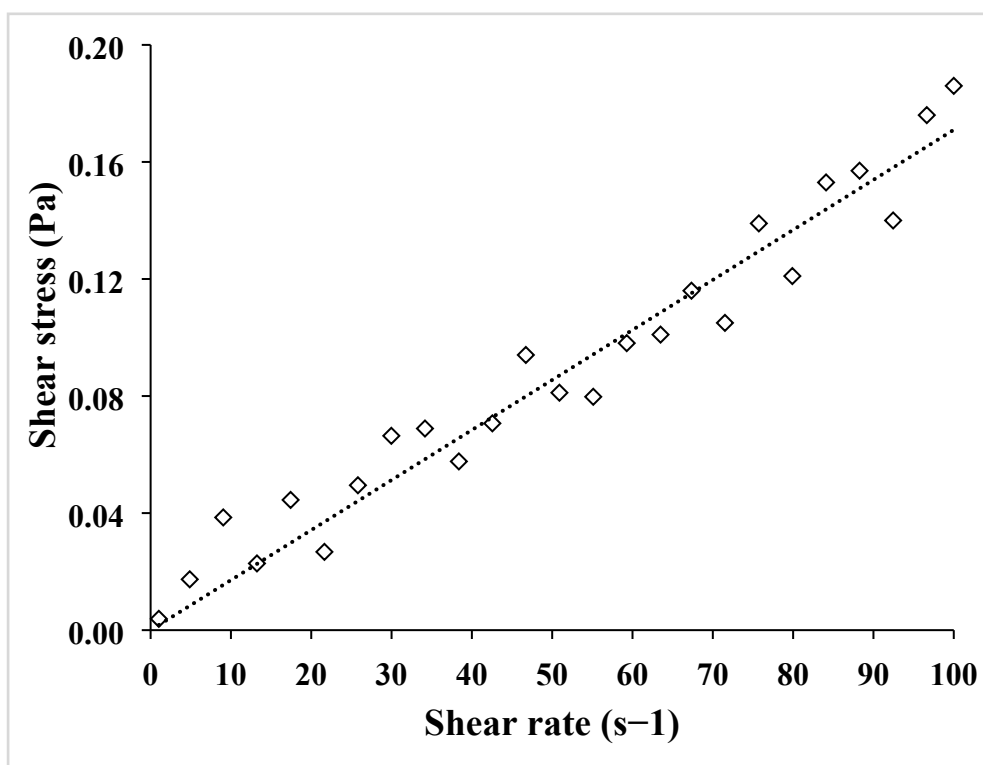
Fig. S1. Flow behavior of Liposome prepared at 170 bar, 50 °C and 1.5% Tween 80.
