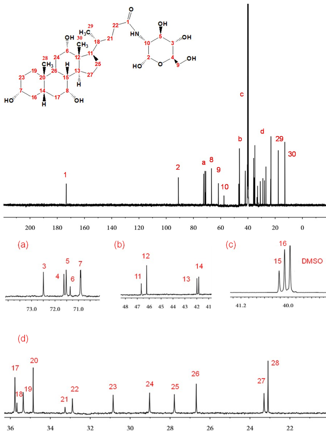
Fig. S1 ^{13}\text{C} -NMR of CAGA, \text{DMSO-}d_6 as solvent.
