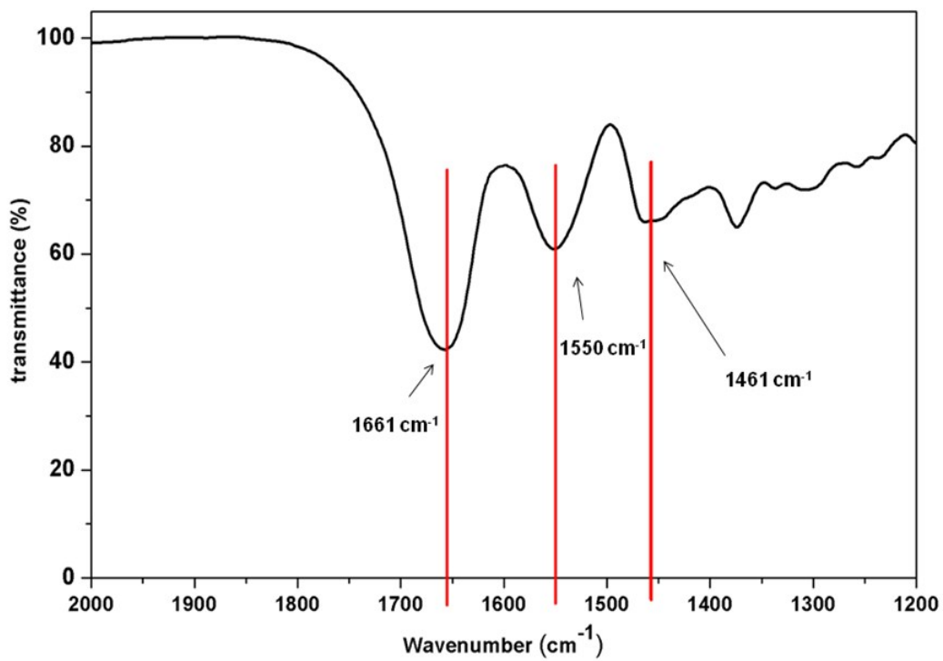
Fig. S2 Partial enlarged FT-IR spectrum of CAGA.
