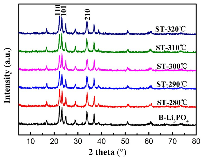
Fig. S1. XRD patterns of Li 3 PO 4 catalysts treated with steam at different temperatures.
