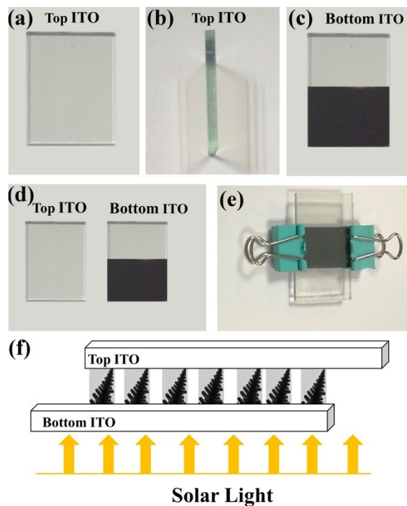
Figure S1. (a) Top-view and (b) side-view optical image of ITO glass; (c) PbS drop-casted on ITO glass; (d) Top-view comparison optical image of ITO glass and PbS/ITO glass; (e) a photoresponse device with ITO/PbS/ITO structure; (f) schematic illustration of the photoresponse device.
