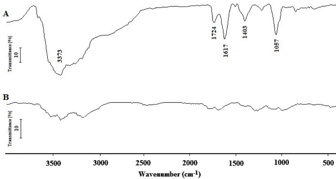
Figure S1. FT-IR spectra of (A) GO and (B) RGO nano sheets.
