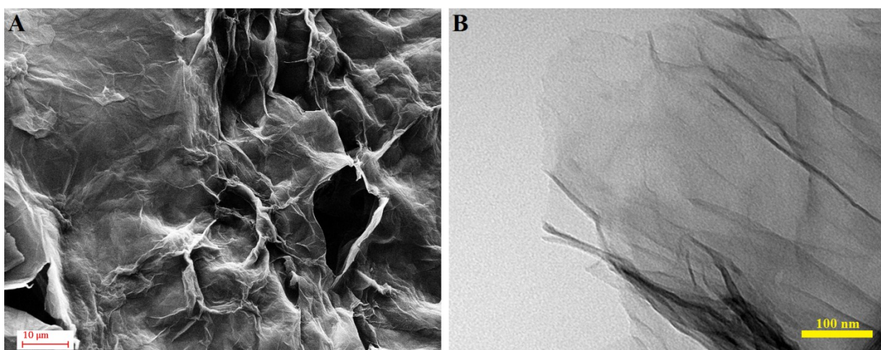
Figure S2. SEM image (A) and TEM image (B) of the prepared RGO nano sheets.
