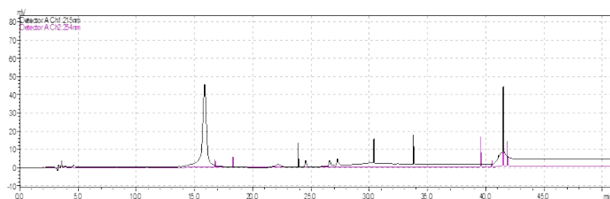
Fig. S2 HPLC figure of 5g/L product isolated from Streptomyces sp. DES20 with hydrochloric acid elution
