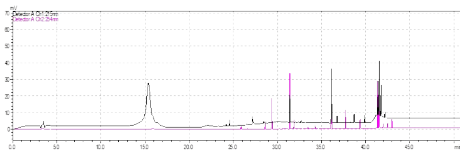
Fig S1 HPLC figure of 5g/L \epsilon -PL standard
