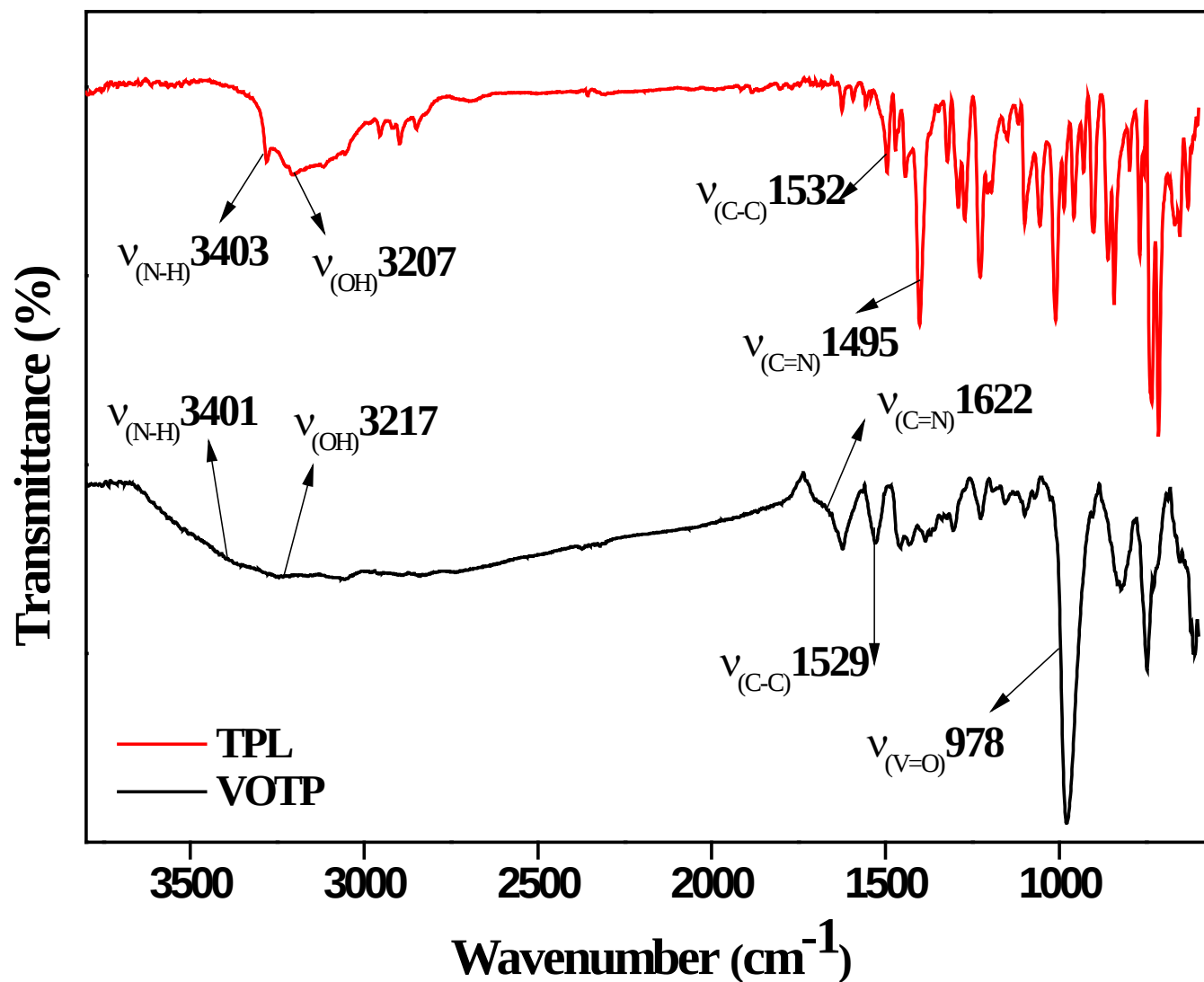
Fig. S3: IR spectrum of TPL and VOTP
