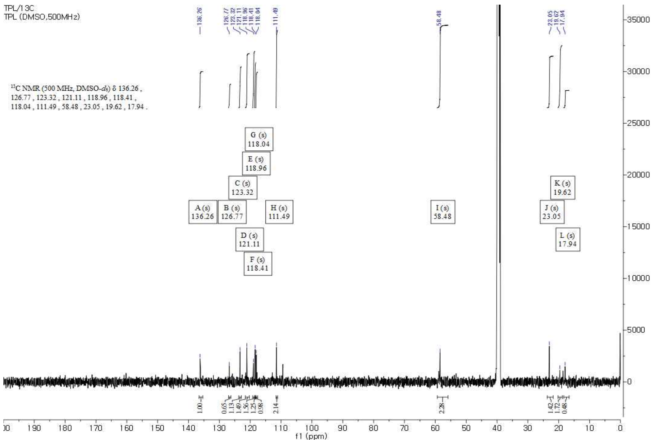
Fig. S5: ^{13}\text{C} NMR spectrum of TPL
