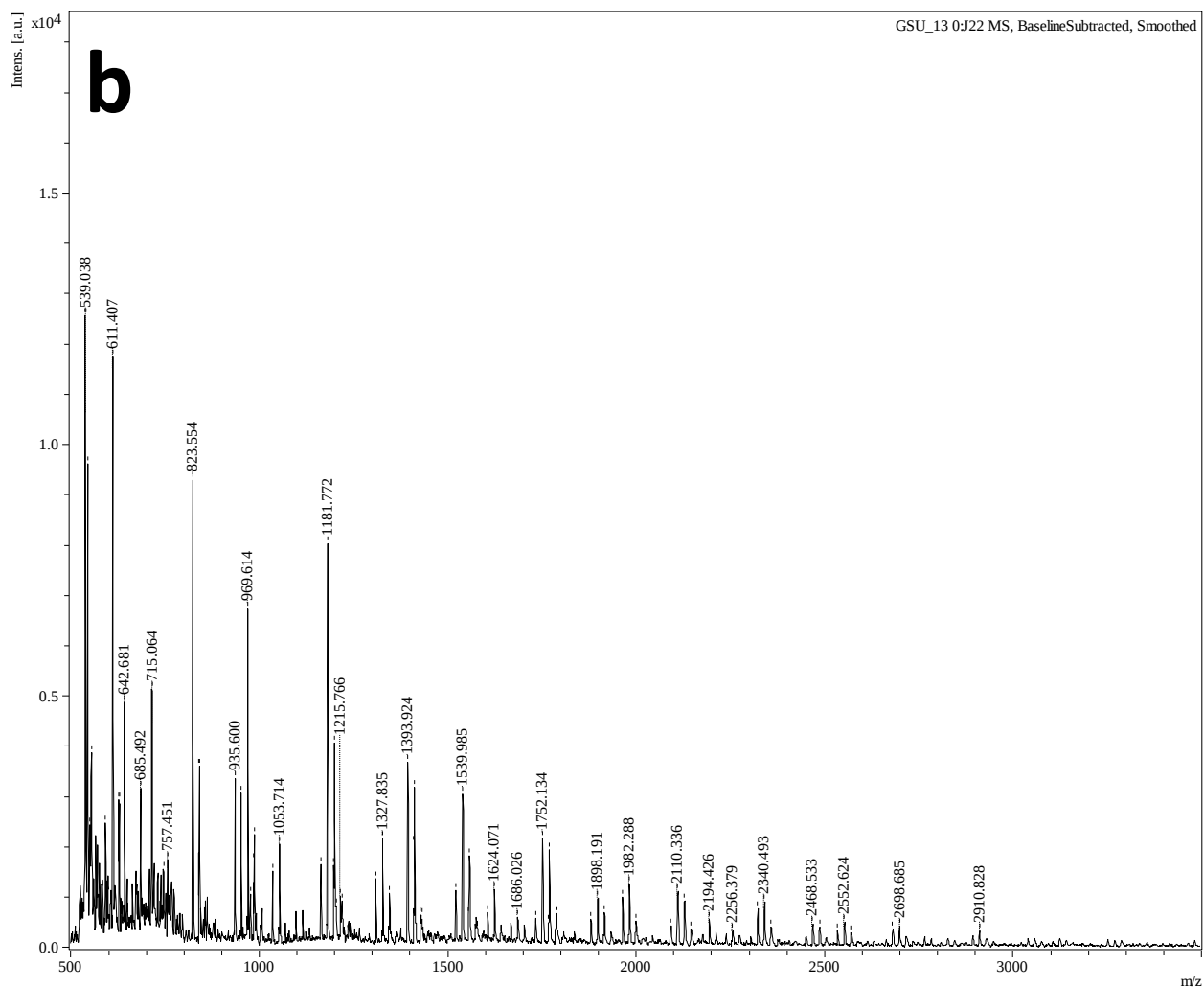
Figure S1 b. MALDI TOF MS spectra of the prepolymer of PGSu 13
