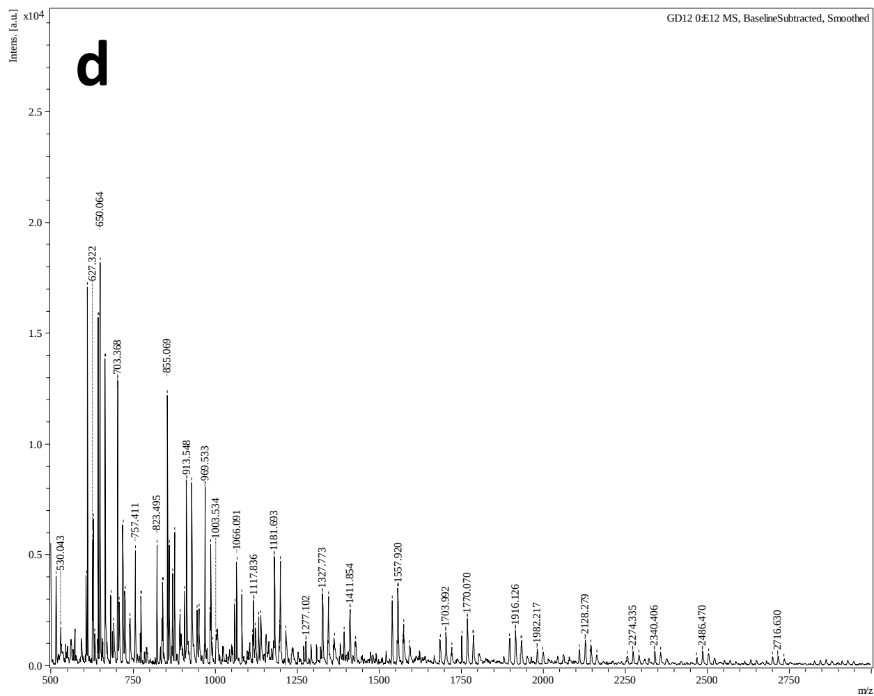
Figure SI d. MALDI TOF MS spectra of the prepolymer of PGD 12
