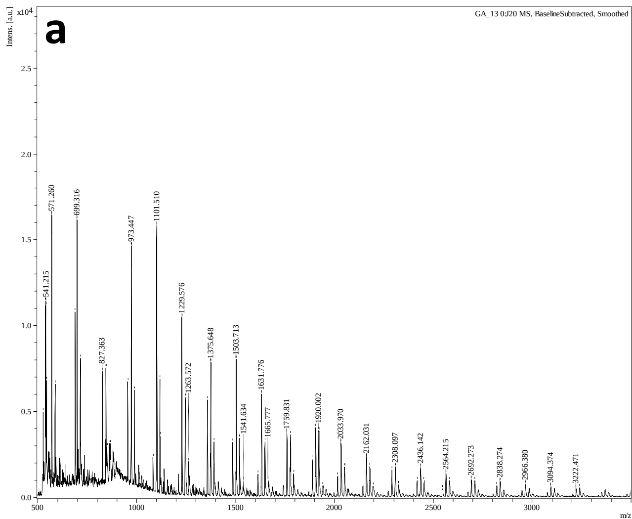
Figure S1 a. MALDI TOF MS spectra of the prepolymer of PGA 13
