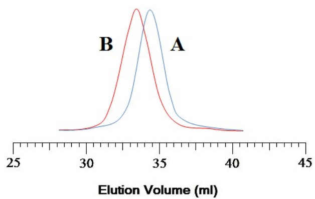
Fig. S2. GPC trace of polymers: FA-PEG- b -P(TBACL- co -CL) (A) and FA-PEG- b -P((PTX-SS-CL)- co -CL) (B).
