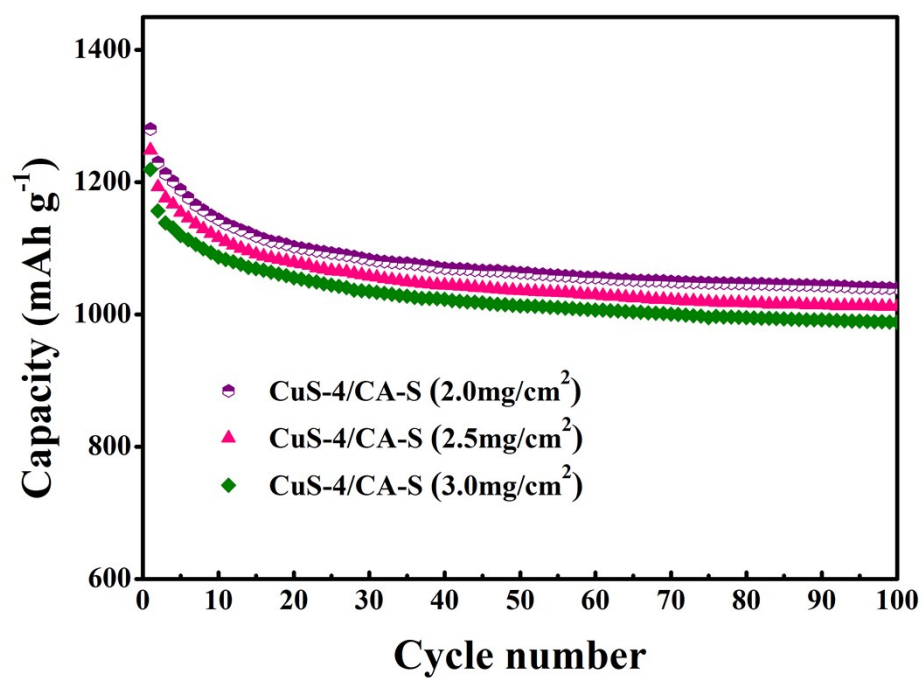
Fig. S2. The cycling performances of CuS-4/CA-S with different sulfur loadings at the rate of 0.2 C.
