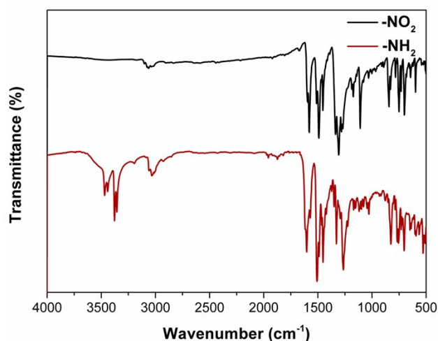
Fig. S1 FTIR spectra of dinitro intermediate compound 1 and diamine monomer 2.
