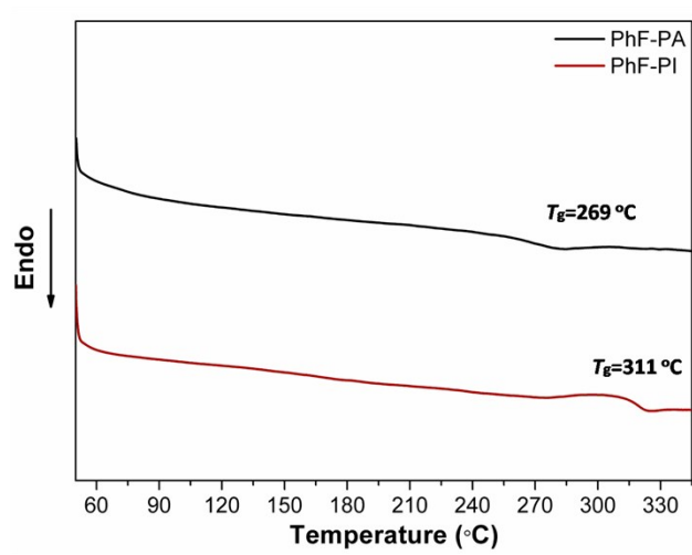
Fig. S4 DSC curves of the polymers.
