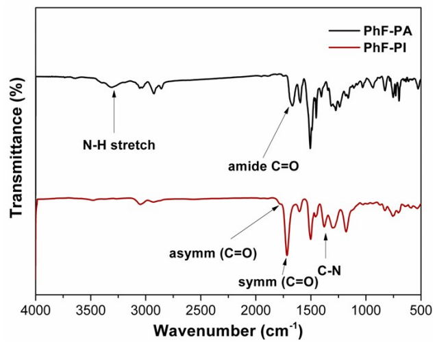
Fig. S2 FTIR spectra of the polymers.
