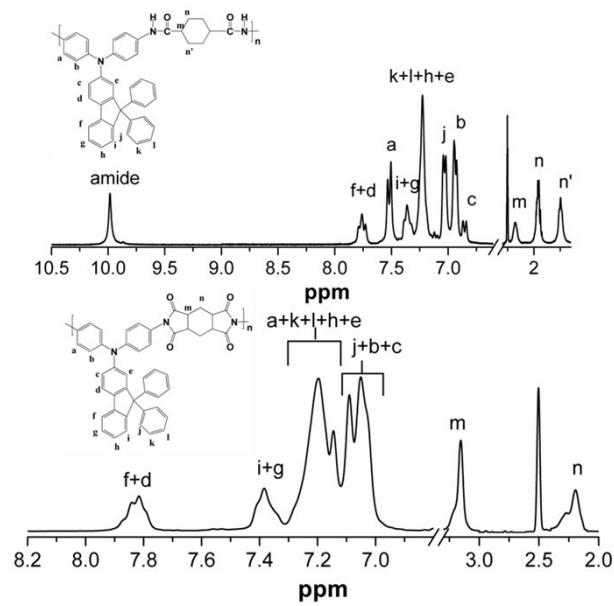
Fig.S3 ^1\text{H} NMR spectra of the polymers in \text{DMSO-}d_6
