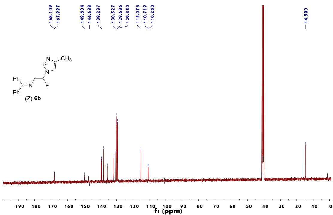
Figure 14. 13 C NMR spectrum of (Z)-6b
