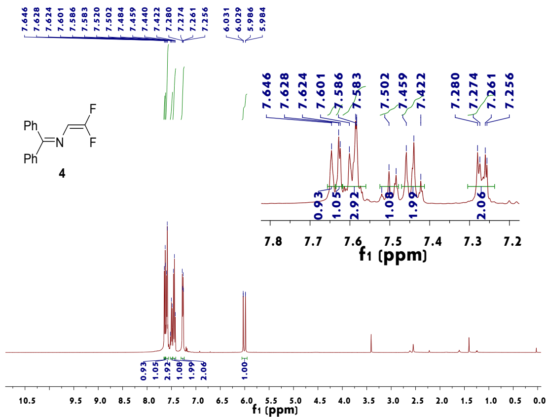
Figure 3. 1 H NMR spectrum of 4
