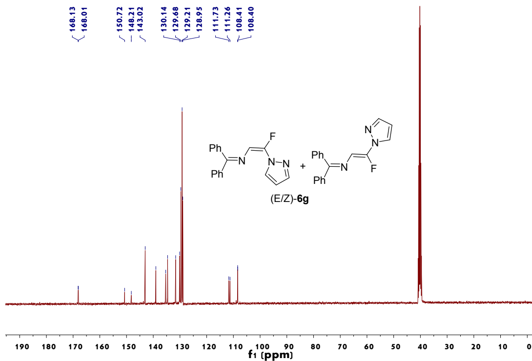
Figure 29. 13 C NMR spectrum of (E/Z)-6g
