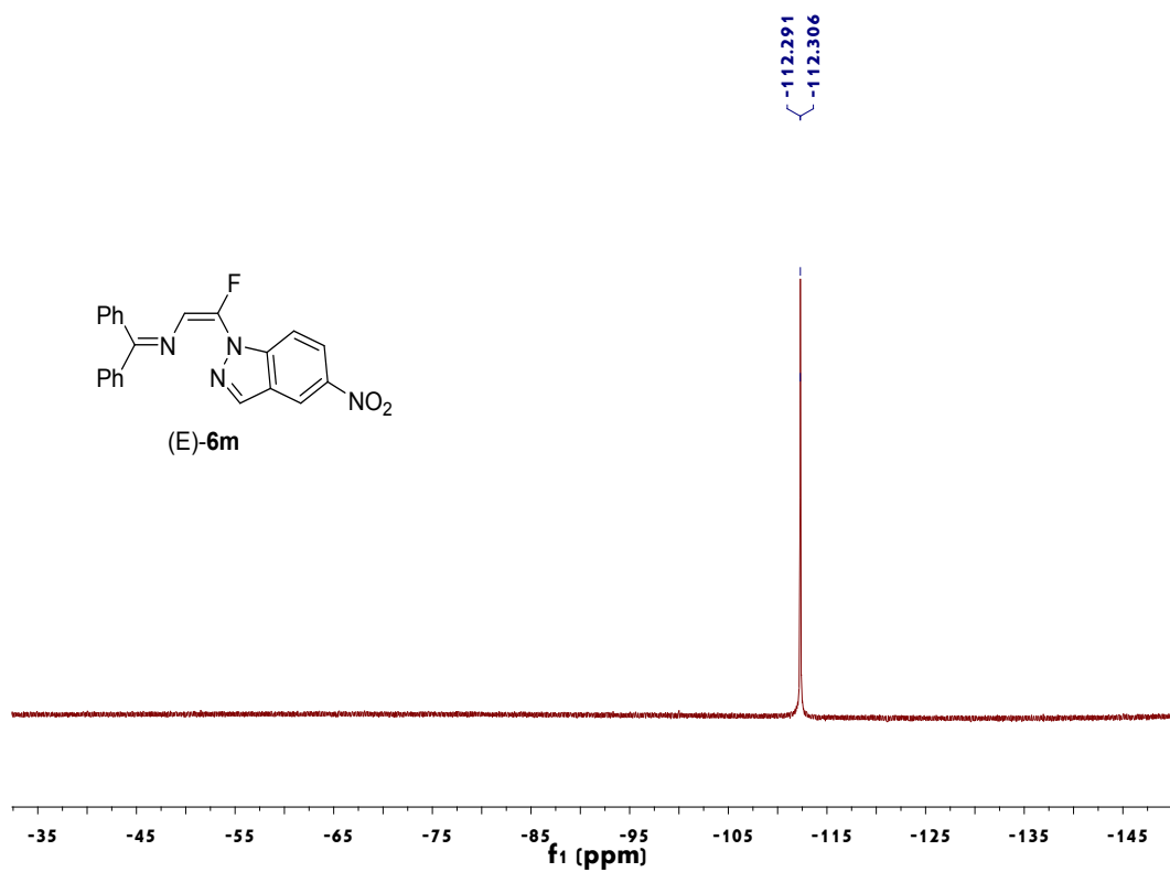
Figure 55. 19 F NMR spectrum of (E)-6m
