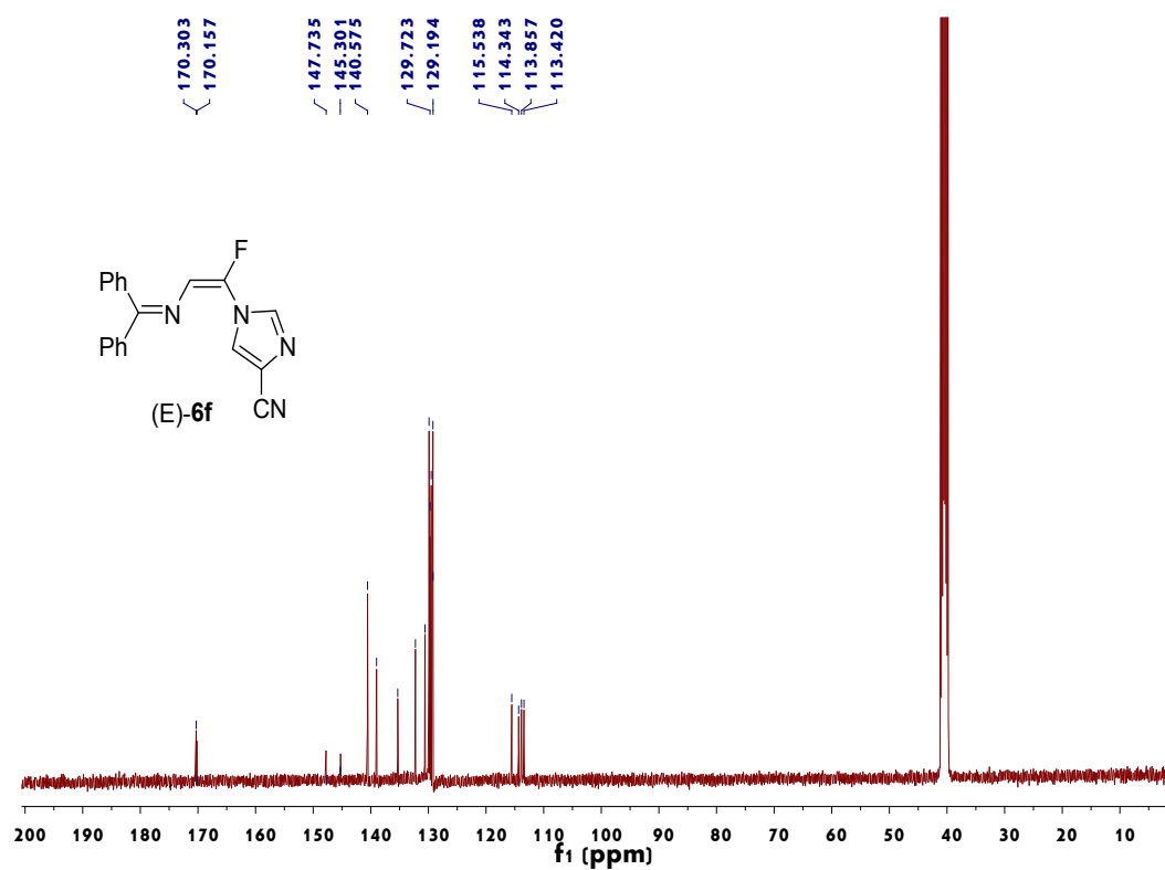
Figure 26. 13 C NMR spectrum of (E)-6f
