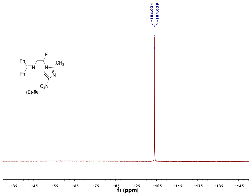
Figure 22. 19 F NMR spectrum of (E)-6e
