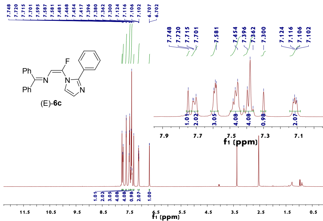
Figure 15. 1 H NMR spectrum of ( E )-6c
