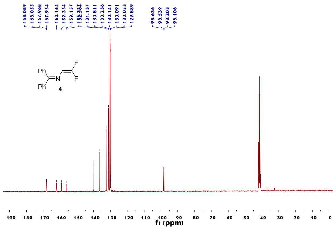
Figure 5. 13 C NMR spectrum of 4
