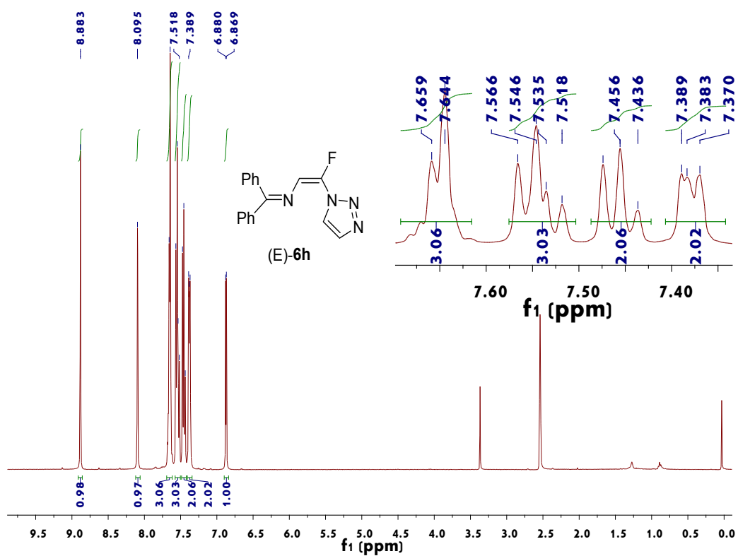
Figure 30. 1 H NMR spectrum of (E)-6h
