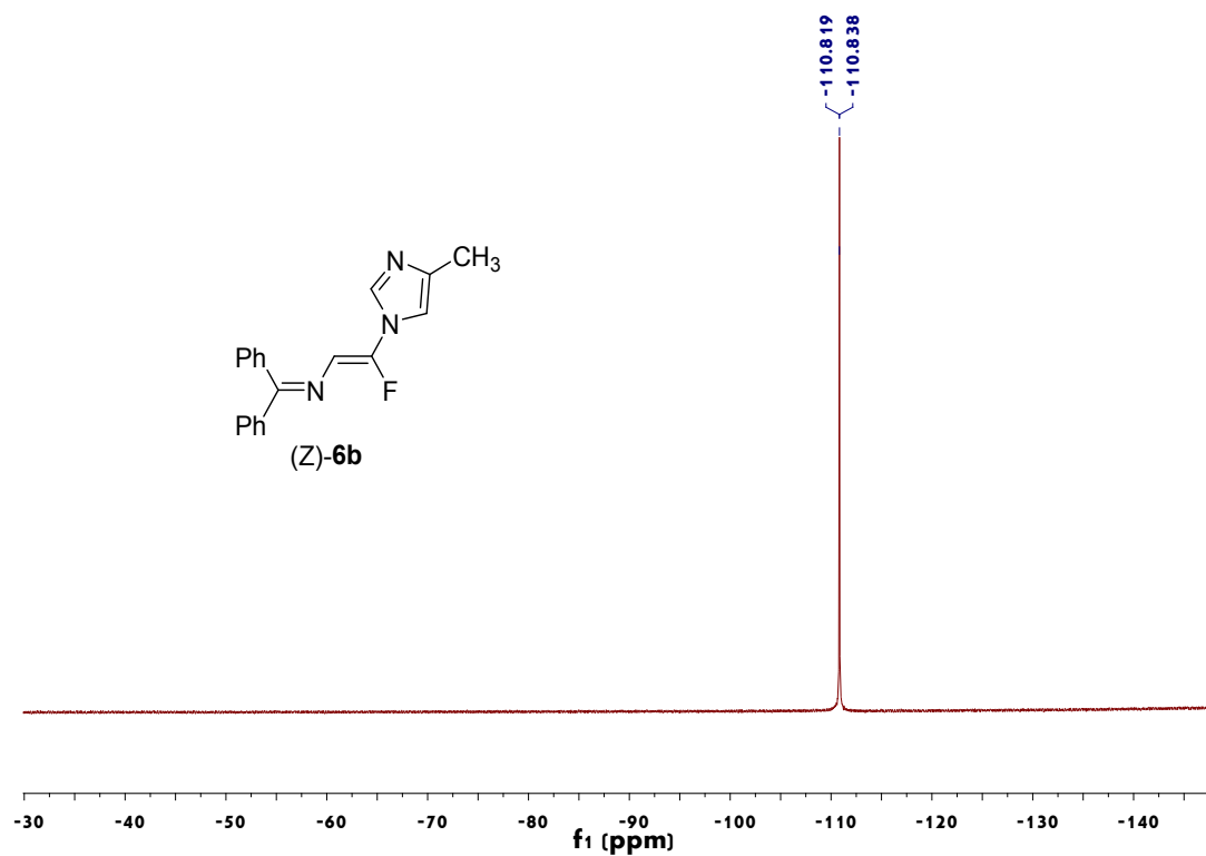
Figure 13. 19 F NMR spectrum of (Z)-6b
