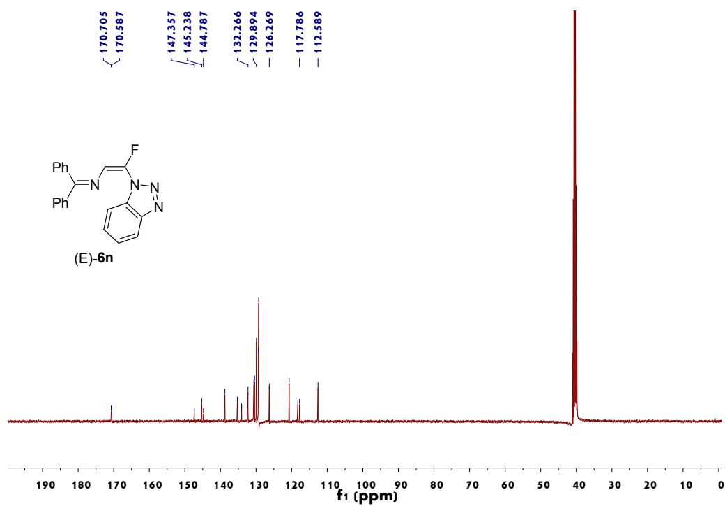
Figure 62. ^{13}\text{C} NMR spectrum of (E)-6n
