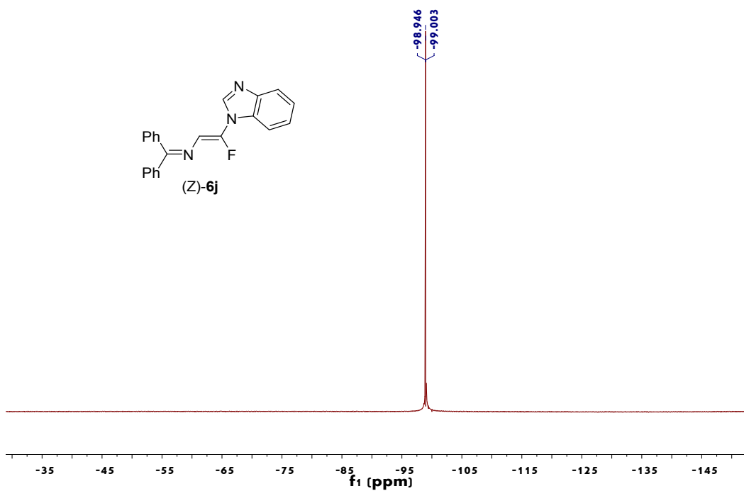
Figure 46. 19 F NMR spectrum of (Z)-6j
