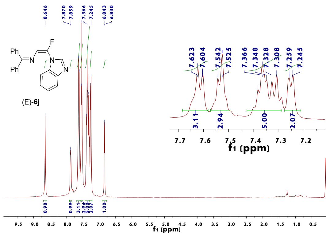
Figure 42. 1 H NMR spectrum of (E)-6j
