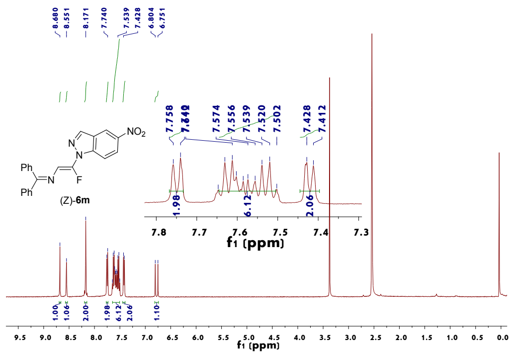
Figure 57. 1 H NMR spectrum of (Z)-6m
