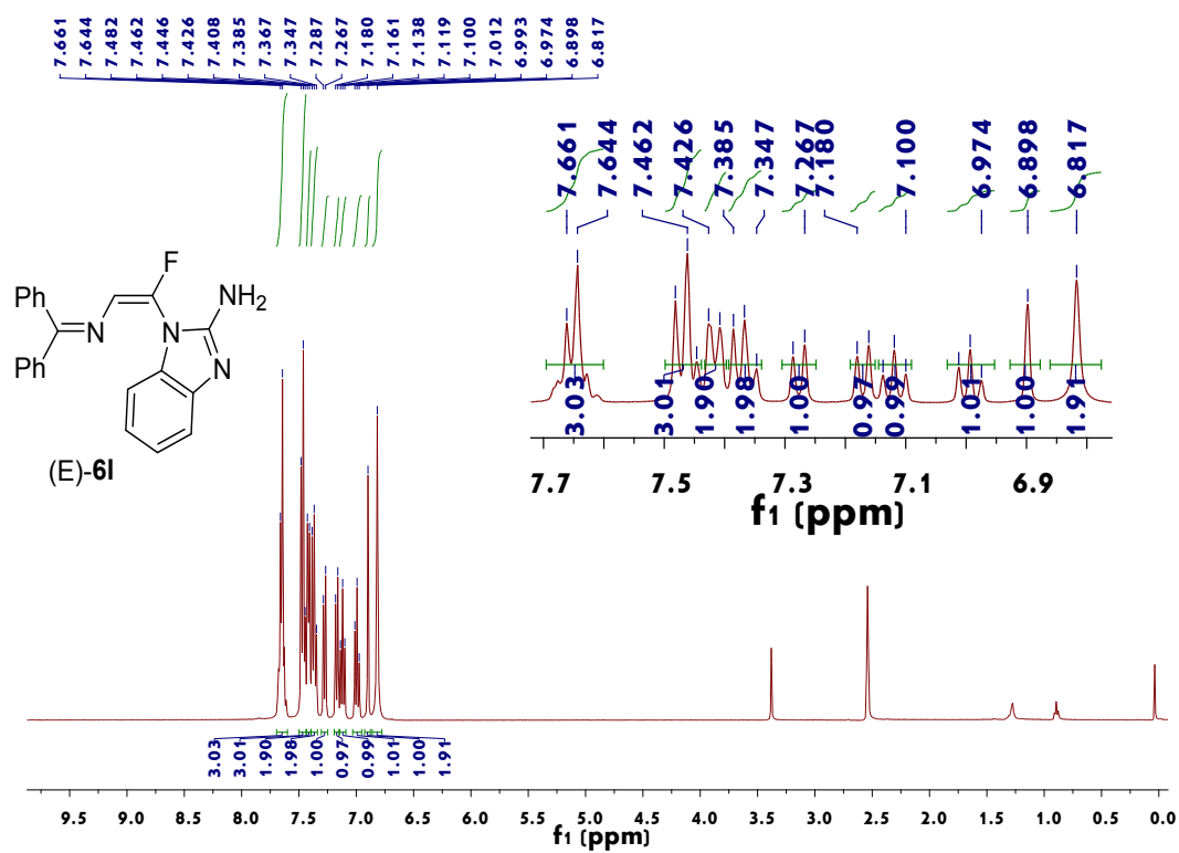
Figure 51. 1 H NMR spectrum of (E)-6I
