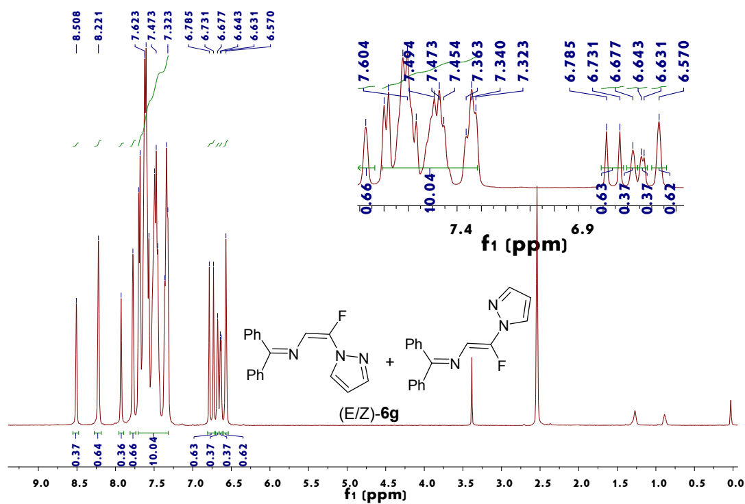
Figure 27. 1 H NMR spectrum of (E/Z)-6g
