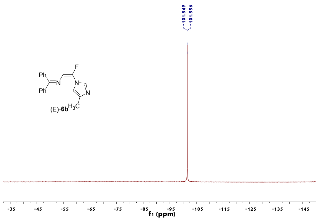
Figure 10. 19 F NMR spectrum of (E)-6b
