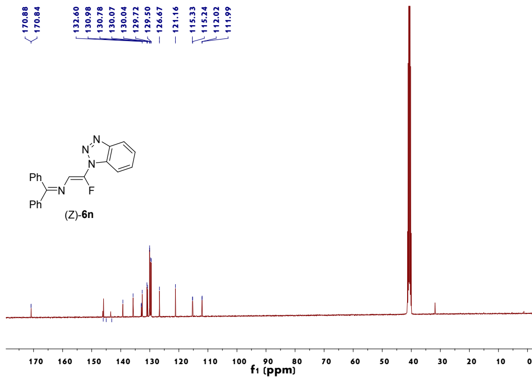
Figure 65. 13 C NMR spectrum of (Z)-6n
