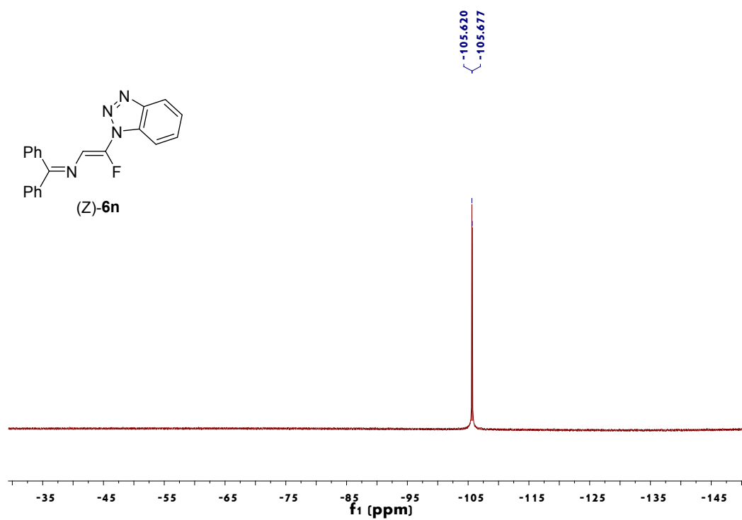
Figure 64. 19 F NMR spectrum of (Z)-6n
