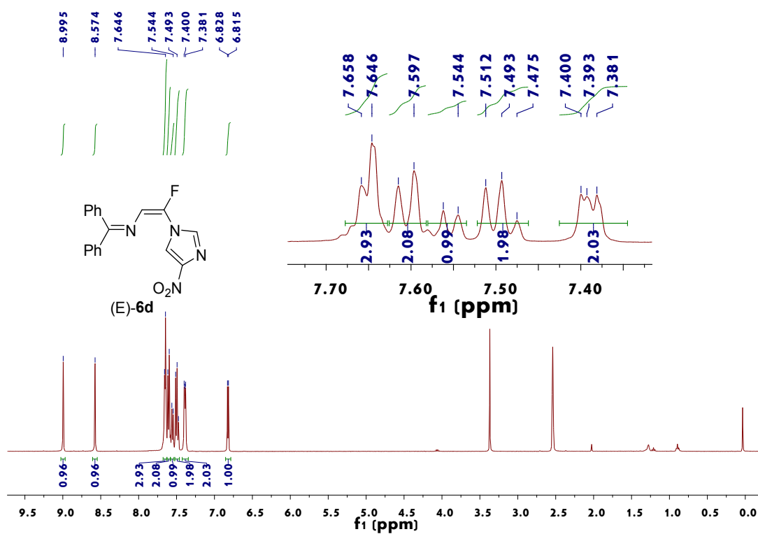
Figure 18. ^1\text{H} NMR spectrum of (E)-6d
