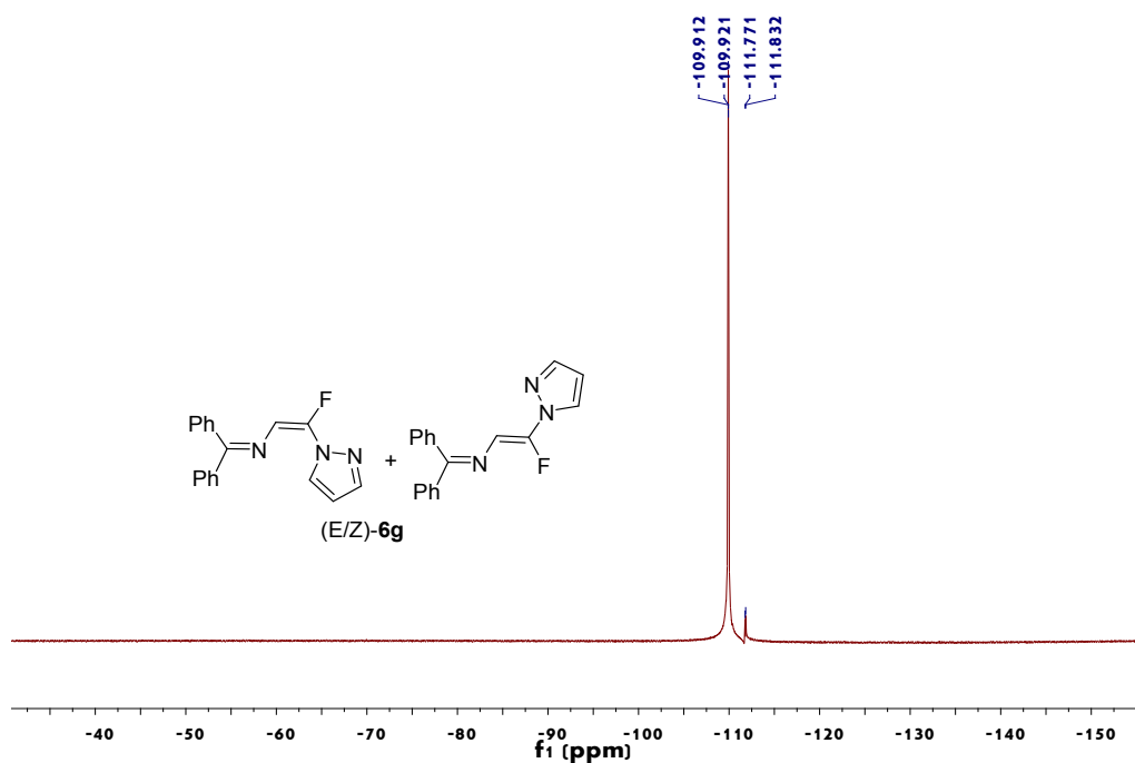
Figure 28. 19 F NMR spectrum of (E/Z)-6g
