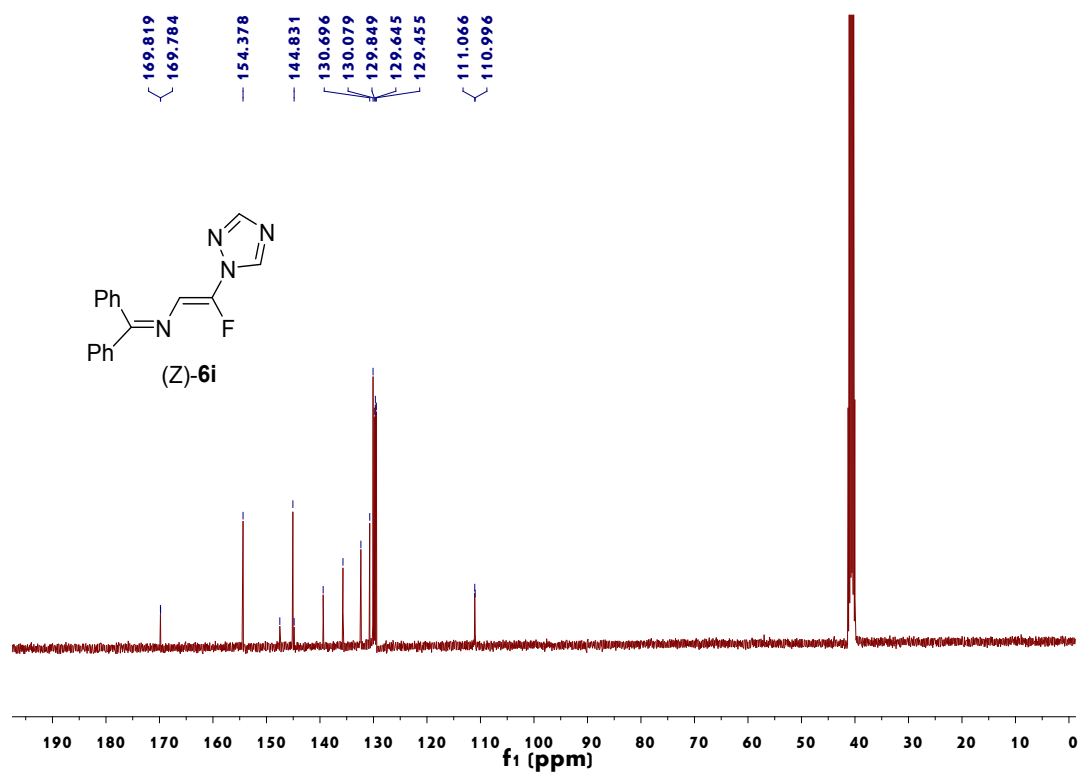
Figure 41. 13 C NMR spectrum of (Z)-6i
