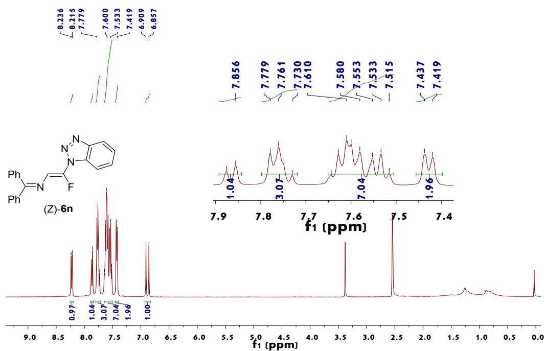
Figure 63. 1 H NMR spectrum of (Z)-6n
