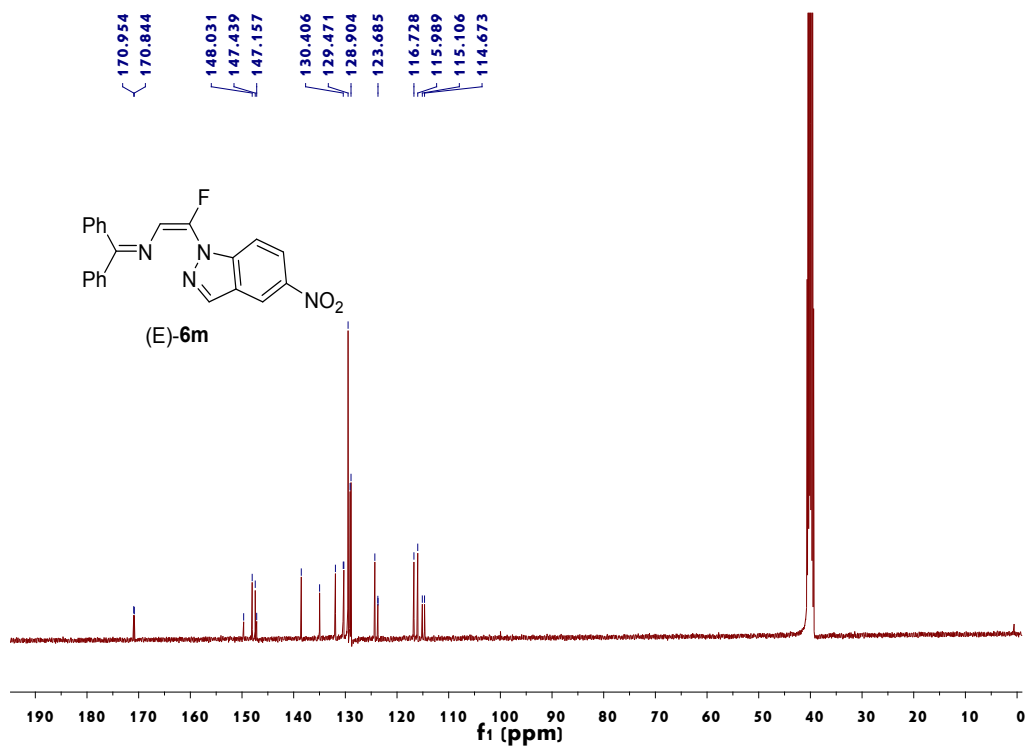
Figure 56. 13 C NMR spectrum of (E)-6m
