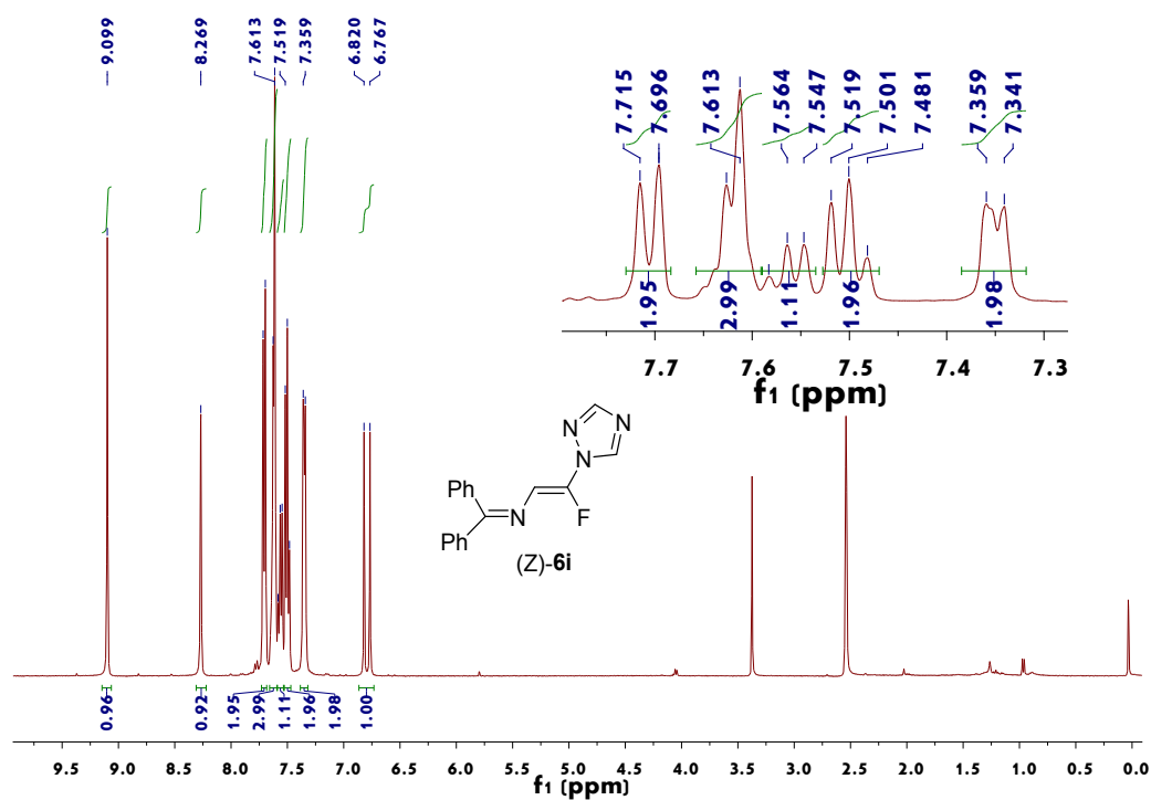
Figure 39. 1 H NMR spectrum of (Z)-6i
