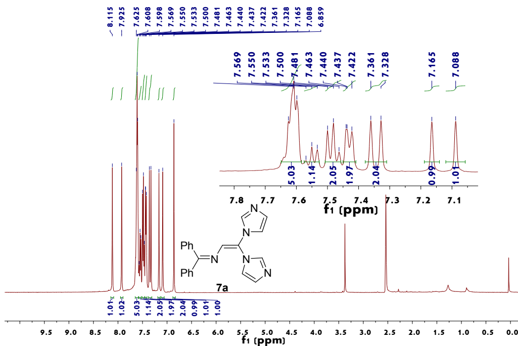
Figure 66. 1 H NMR spectrum of 7a
