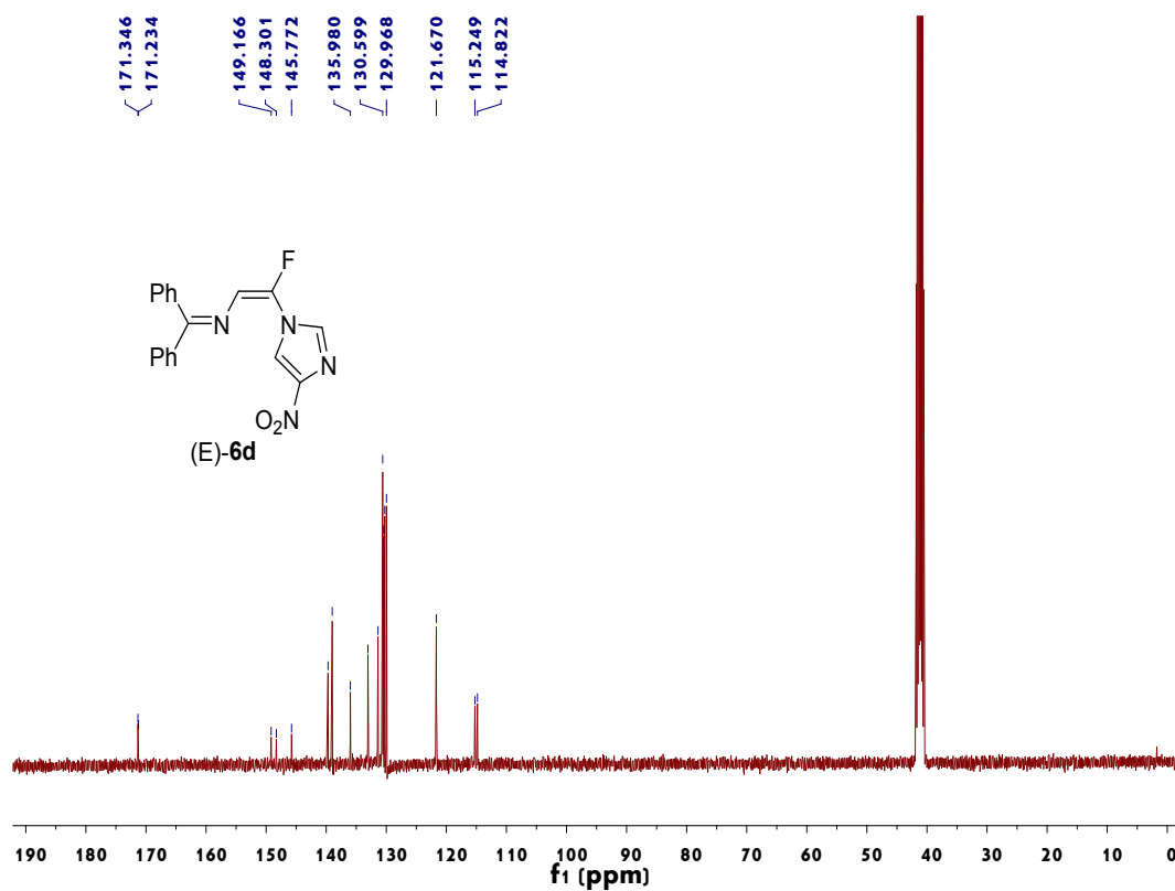
Figure 20. ^{13}\text{C} NMR spectrum of (E)- 6d
