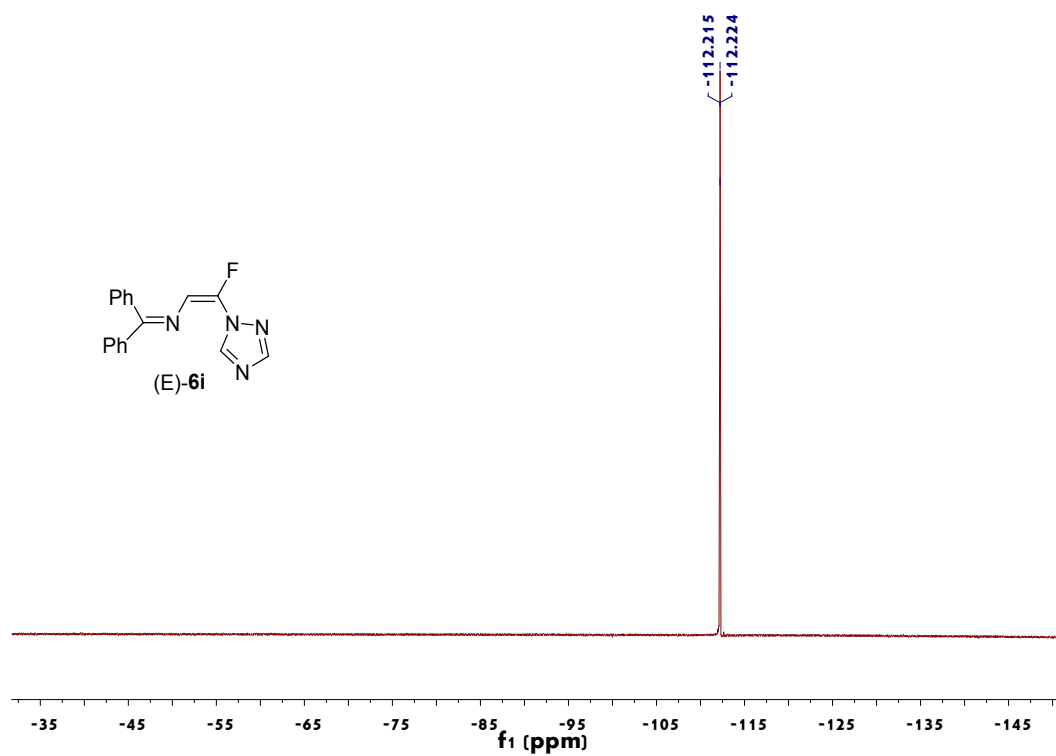
Figure 37. 19 F NMR spectrum of (E)-6i
