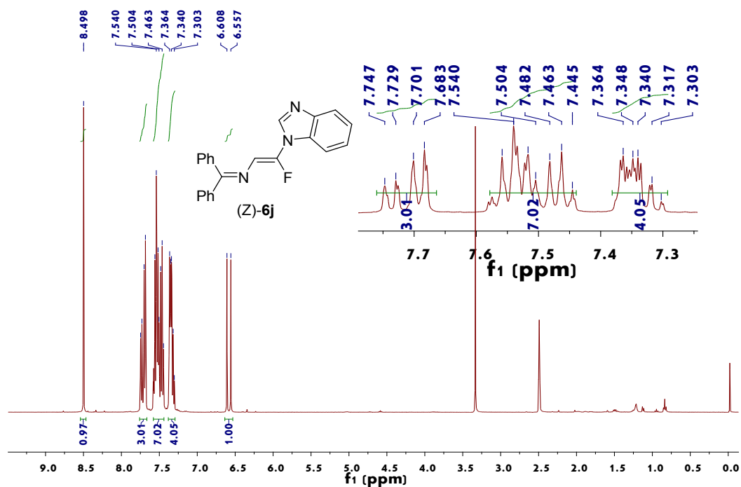
Figure 45. 1 H NMR spectrum of (Z)-6j
