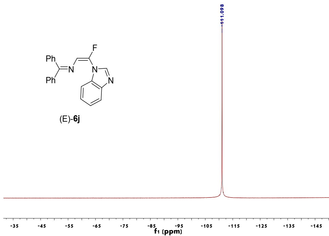
Figure 43. ^{19}\text{F} NMR spectrum of (E)-6j
