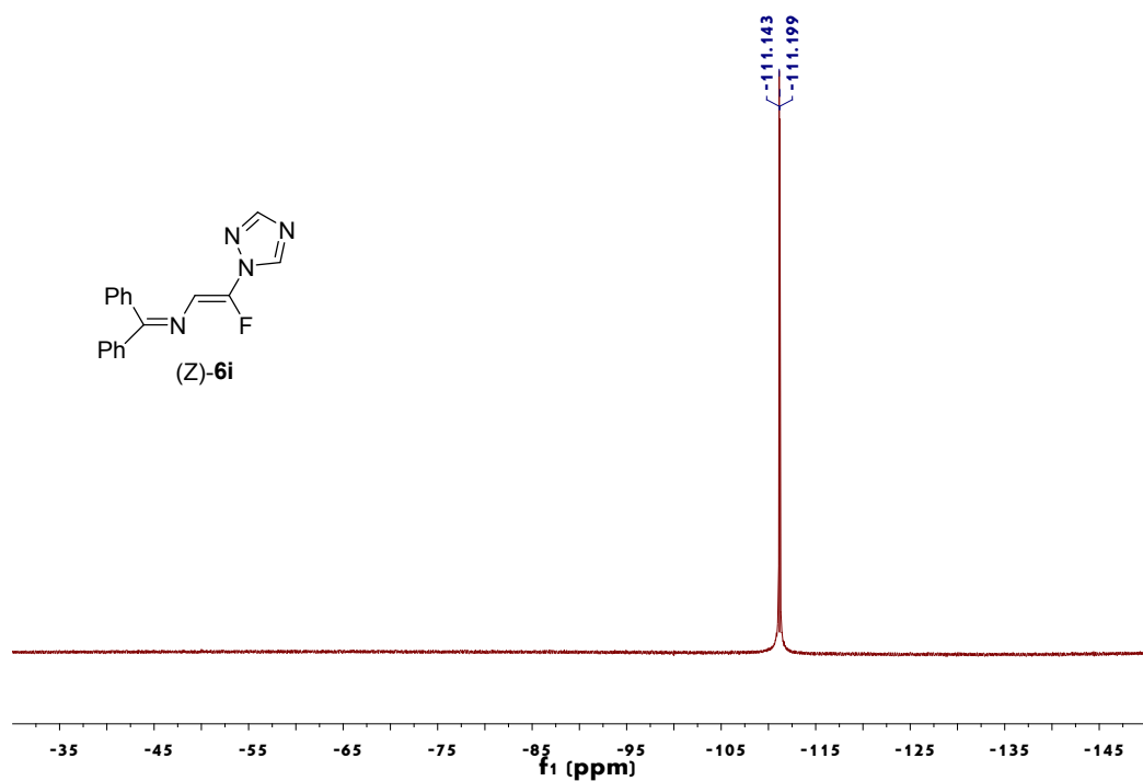
Figure 40. 19 F NMR spectrum of (Z)-6i
