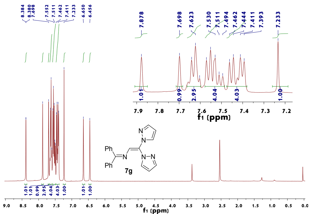
Figure 70. 1 H NMR spectrum of 7g
