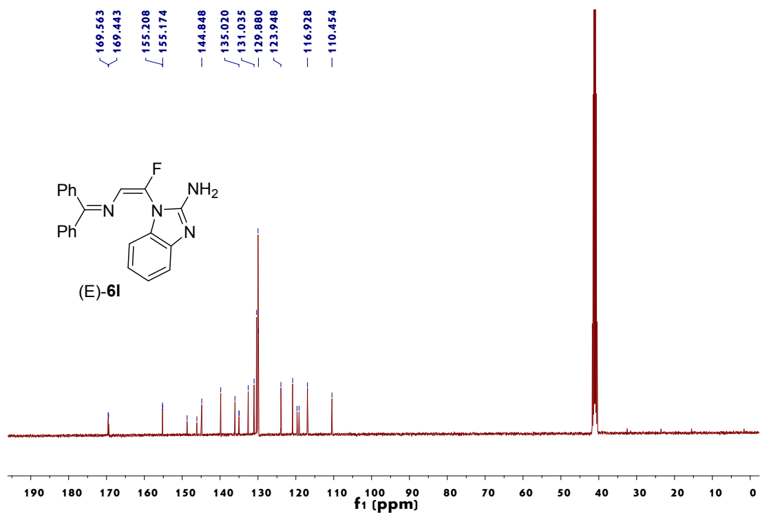
Figure 53. ^{13}\text{C} NMR spectrum of (E)-6l
