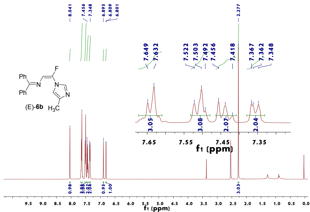
Figure 9. 1 H NMR spectrum of (E)-6b
