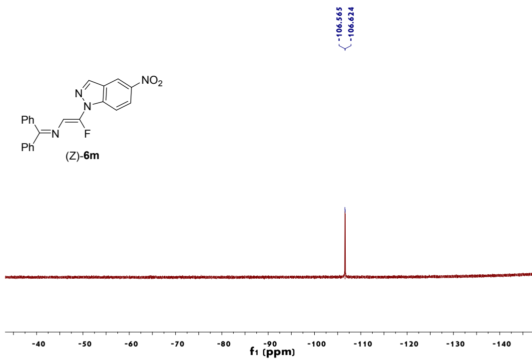
Figure 58. 19 F NMR spectrum of (Z)-6m
