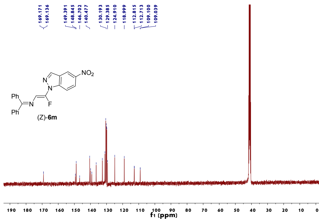
Figure 59. 13 C NMR spectrum of (Z)-6m
