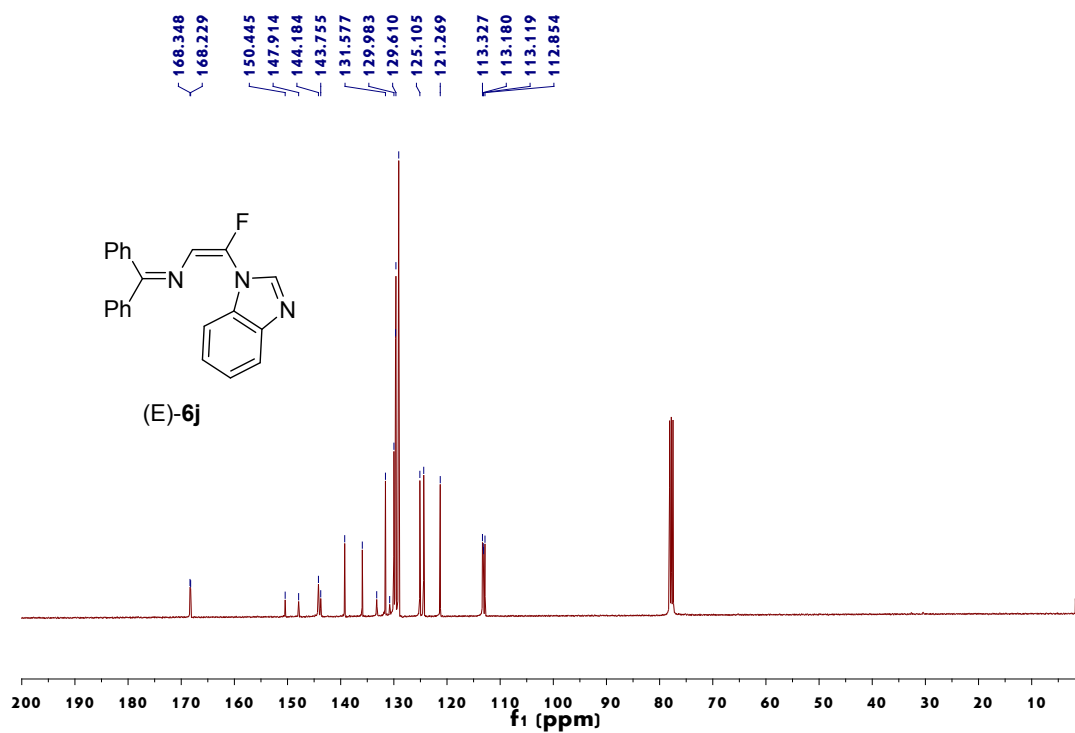
Figure 44. ^{13}\text{C} NMR spectrum of (E)-6j
