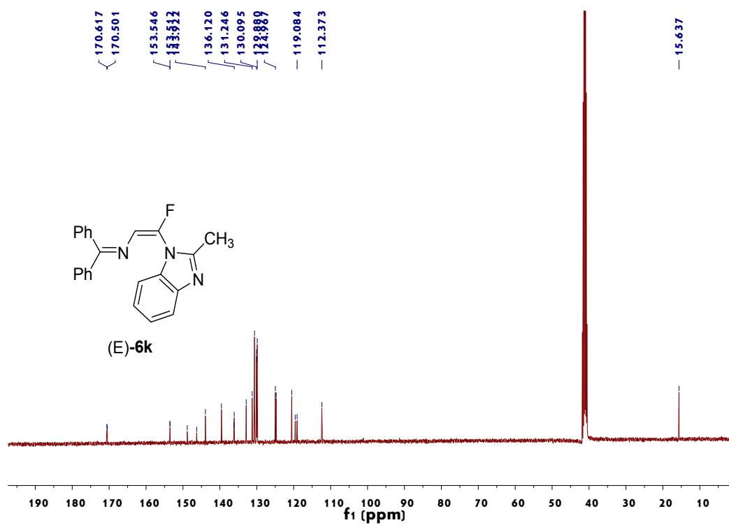
Figure 50. 13 C NMR spectrum of (E)-6k
