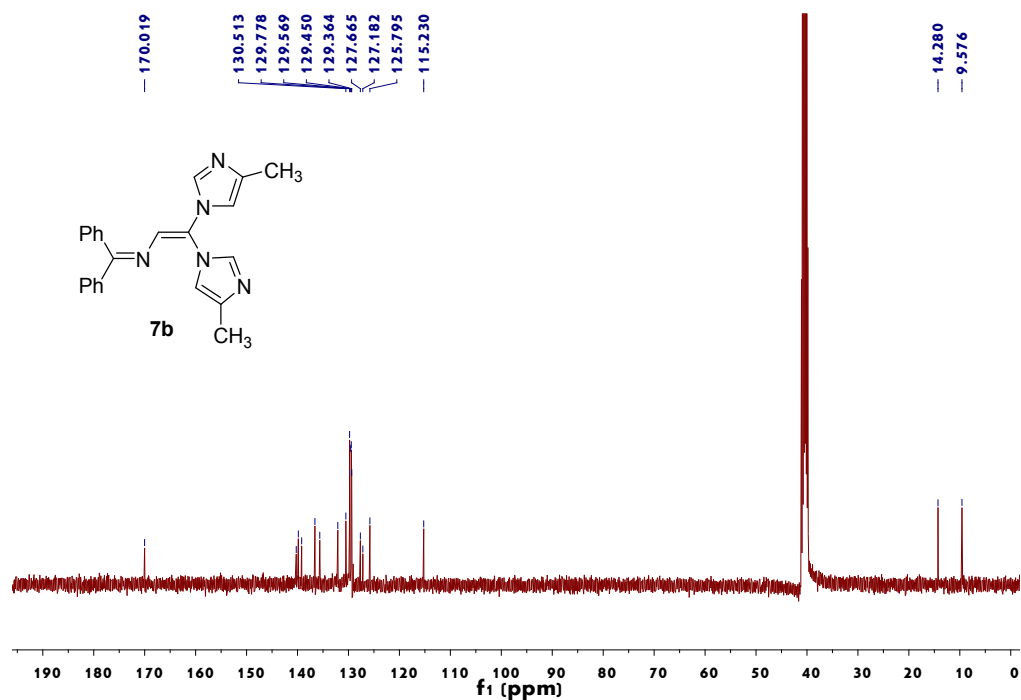
Figure 69. 13 C NMR spectrum of 7b
