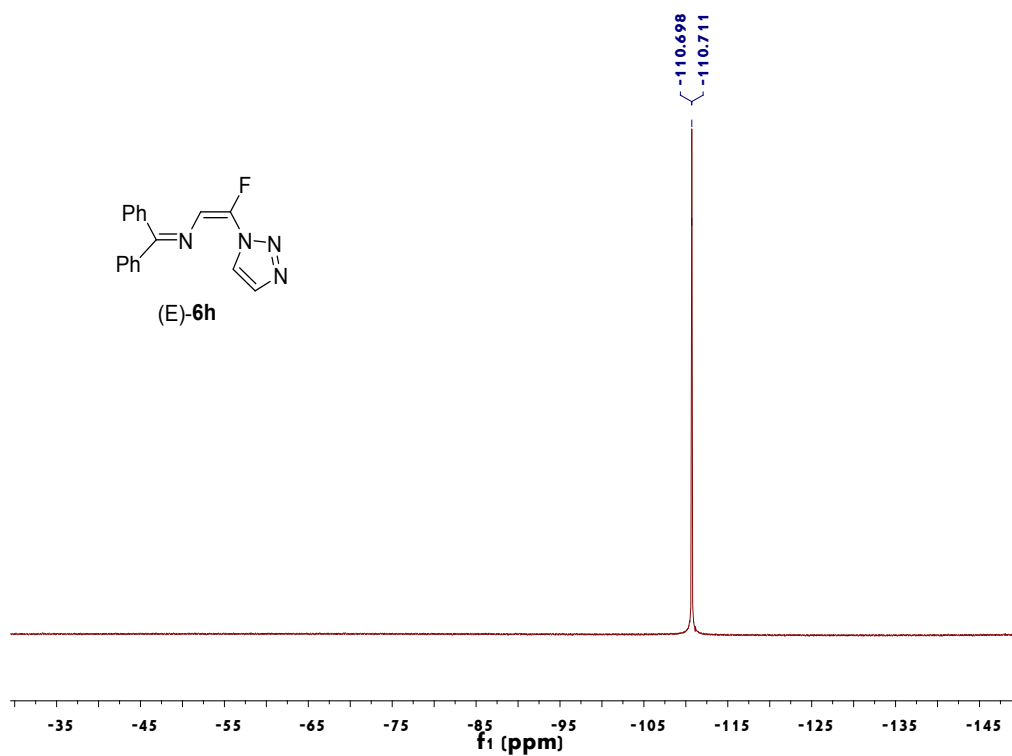
Figure 31. ^{19}\text{F} NMR spectrum of (E)-6h
