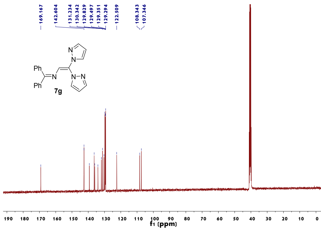
Figure 71. 13 C NMR spectrum of 7g
