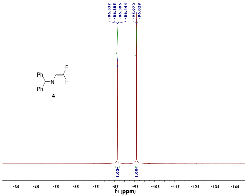
Figure 4. 19 F NMR spectrum of 4
