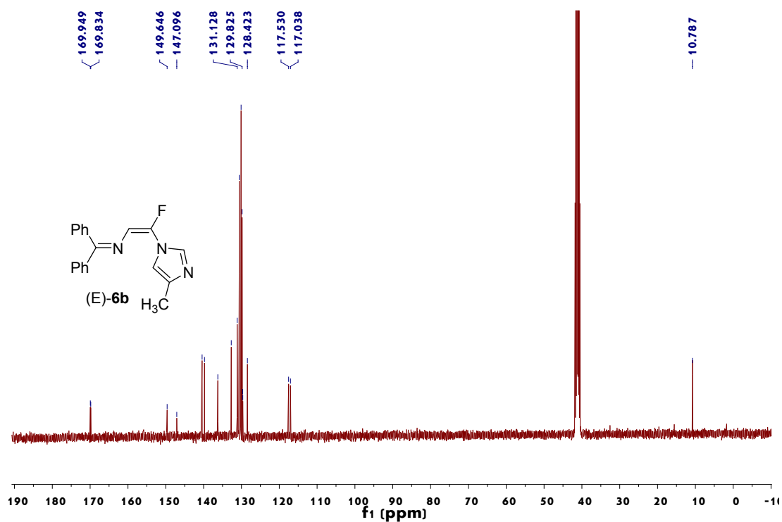
Figure 11. 13 C NMR spectrum of (E)-6b
