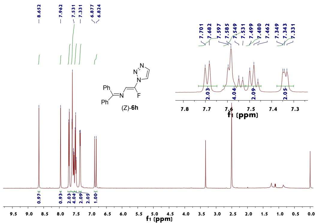
Figure 33. 1 H NMR spectrum of (Z)-6h
