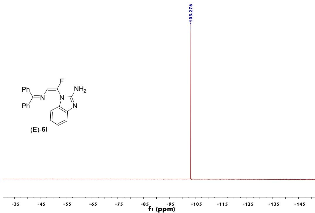
Figure 52. 19 F NMR spectrum of (E)-6I
