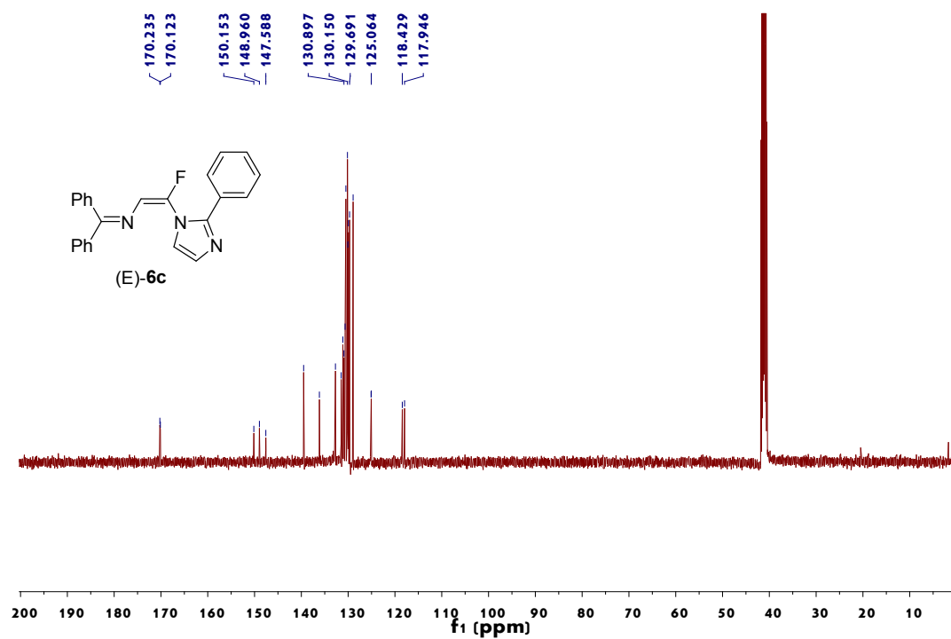
Figure 17. ^{13}\text{C} NMR spectrum of (E)-6c
