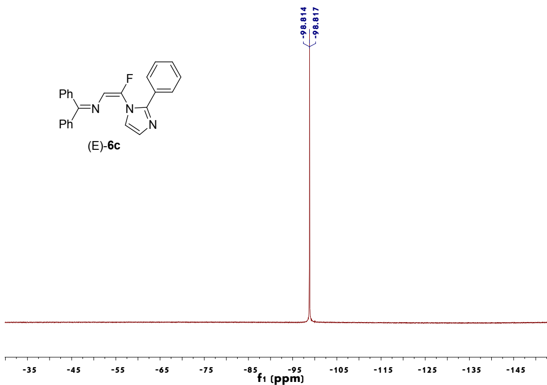
Figure 16. 19 F NMR spectrum of ( E )-6c
