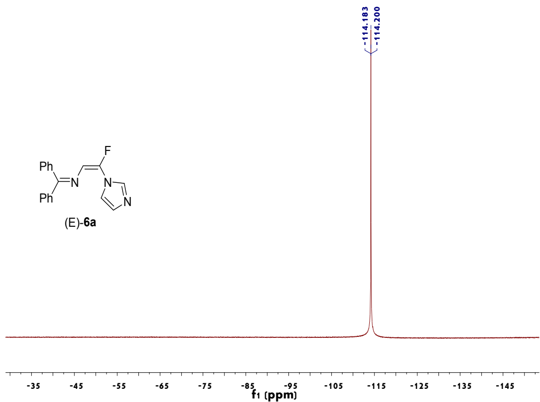
Figure 7. 19 F NMR spectrum of (E)-6a
