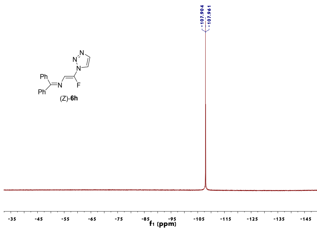
Figure 34. 19 F NMR spectrum of (Z)-6h
