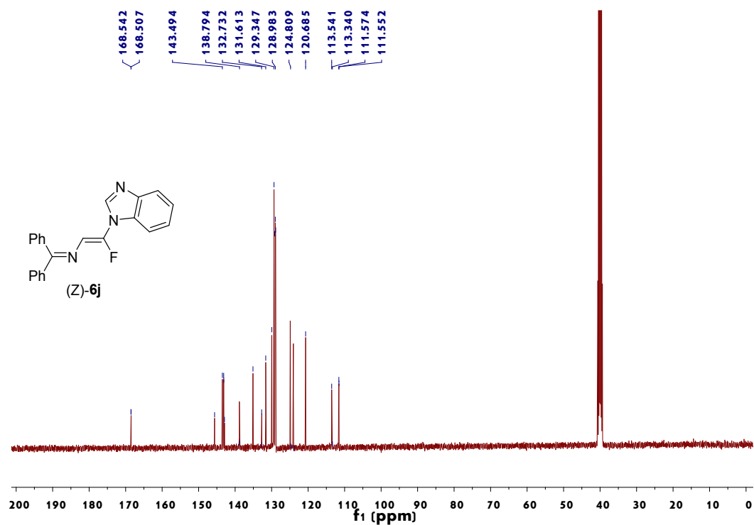
Figure 47. 13 C NMR spectrum of (Z)-6j
