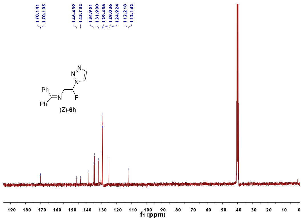
Figure 35. 13 C NMR spectrum of (Z)-6h
