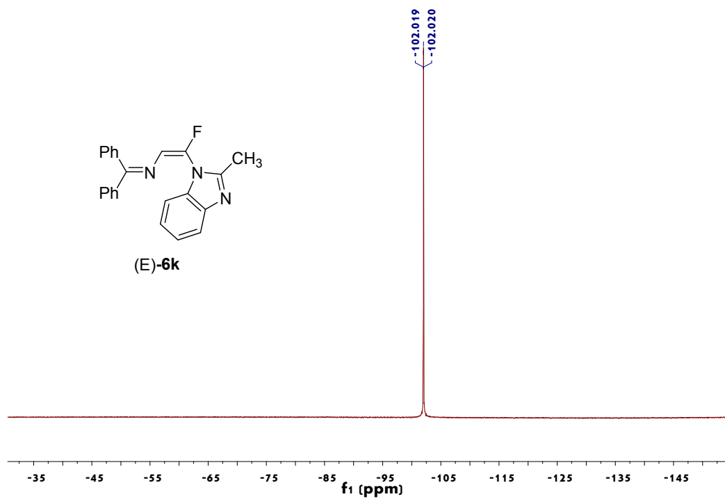
Figure 49. 19 F NMR spectrum of (E)-6k
