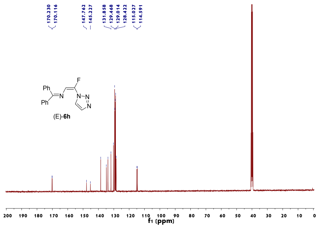
Figure 32. ^{13}\text{C} NMR spectrum of (E)-6h
