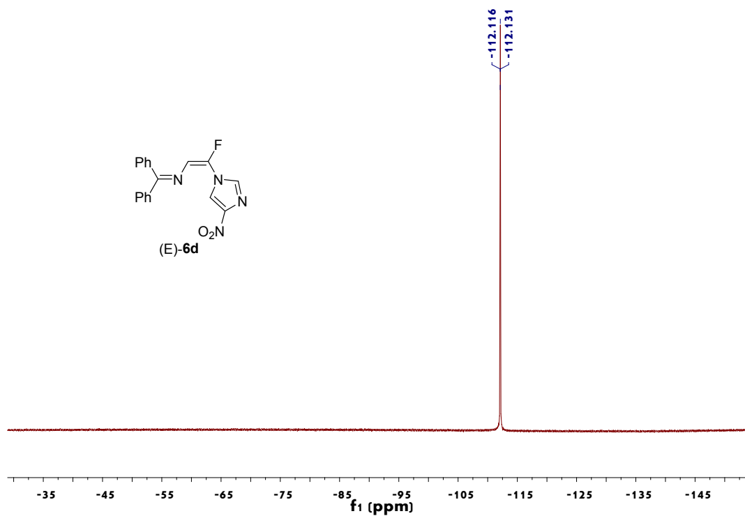
Figure 19. ^{19}\text{F} NMR spectrum of (E)- 6d
