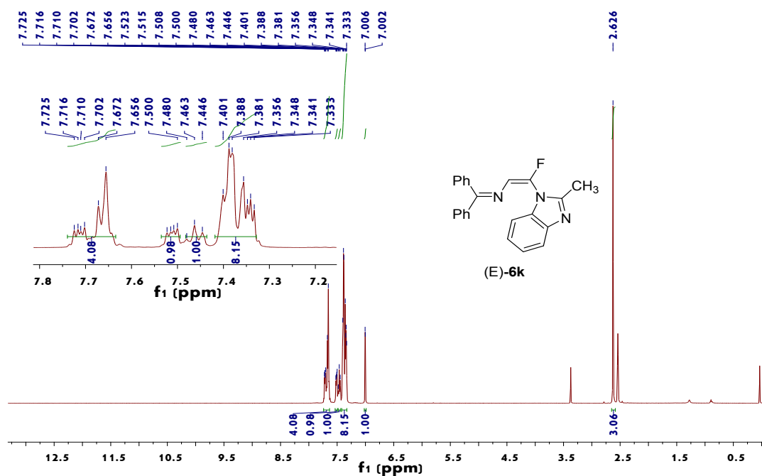
Figure 48. 1 H NMR spectrum of (E)-6k
