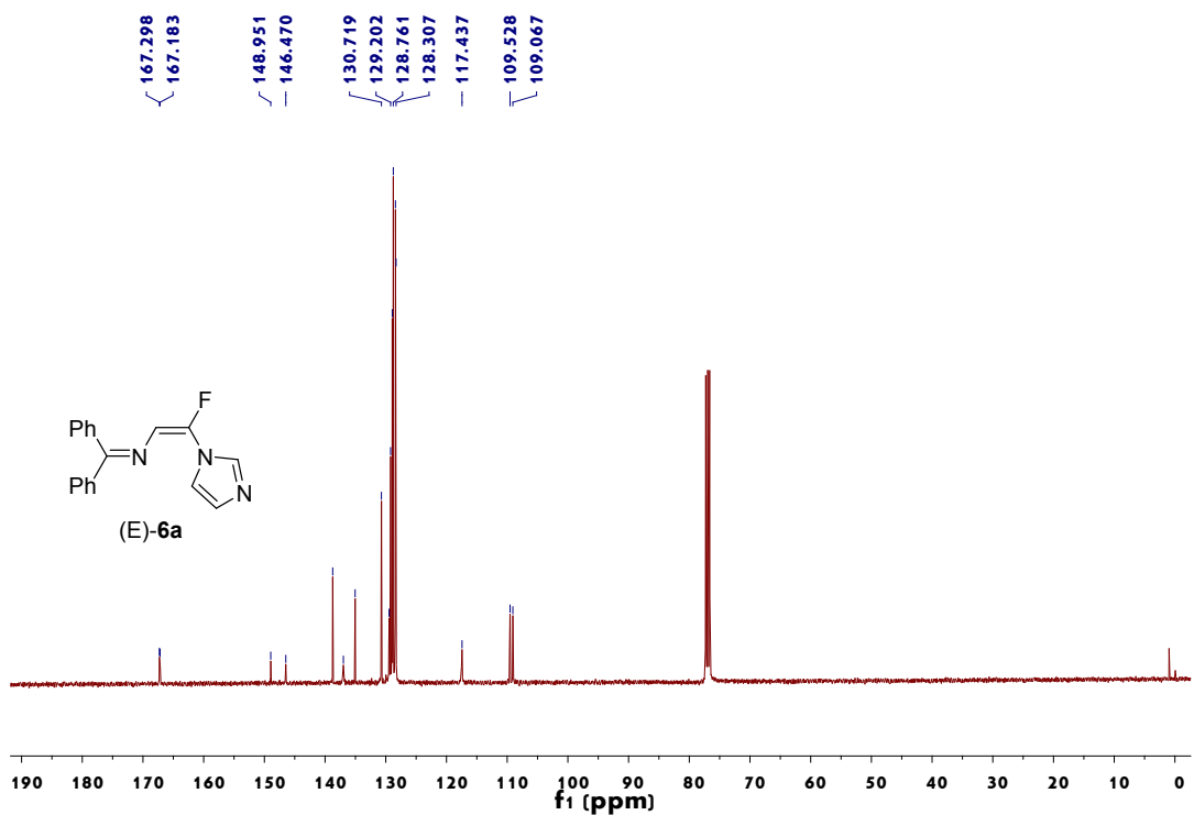
Figure 8. 13 C NMR spectrum of (E)-6a
