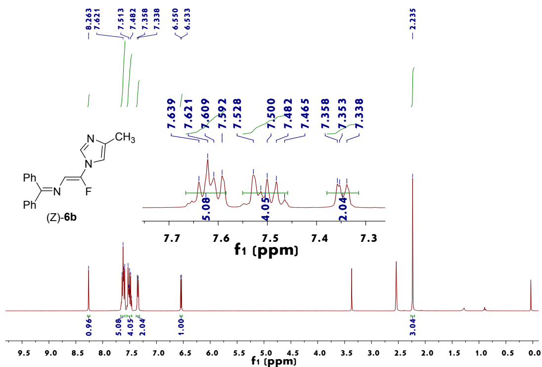
Figure 12. 1 H NMR spectrum of (Z)-6b
