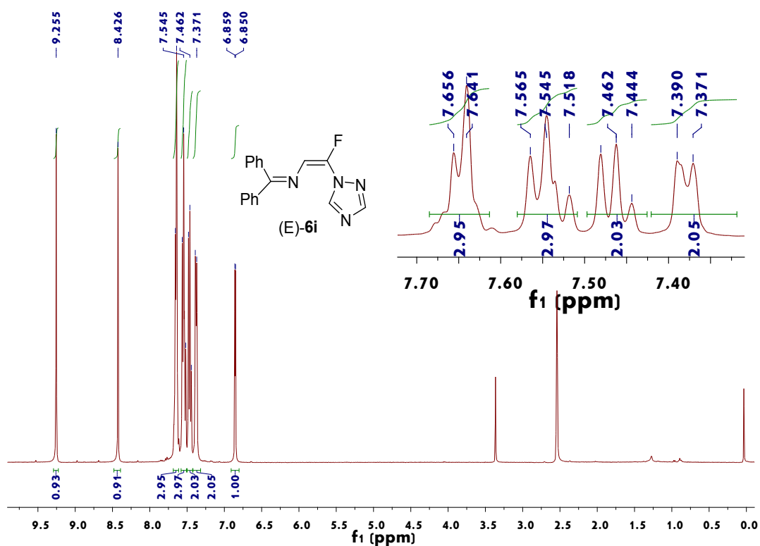
Figure 36. 1 H NMR spectrum of (E)-6i
