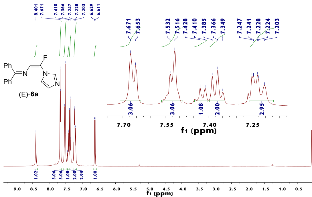
Figure 6. 1 H NMR spectrum of (E)-6a
