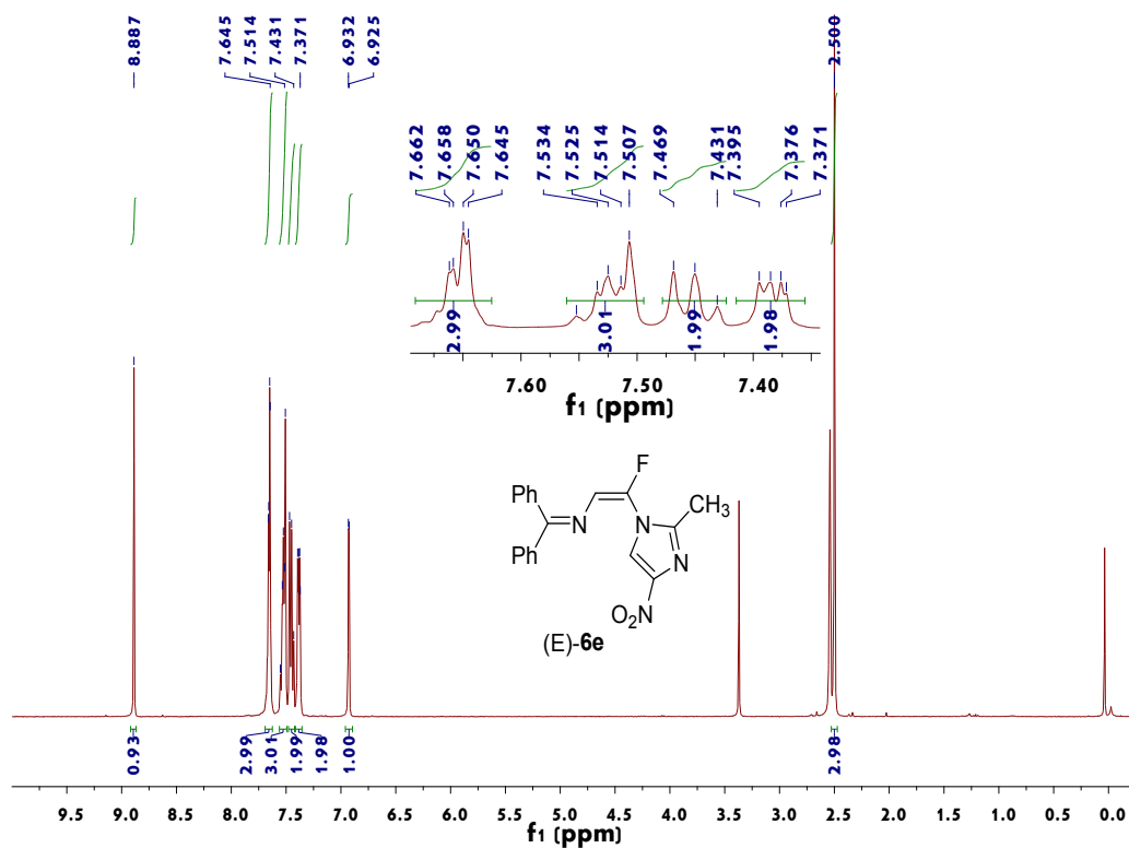
Figure 21. 1 H NMR spectrum of (E)-6e
