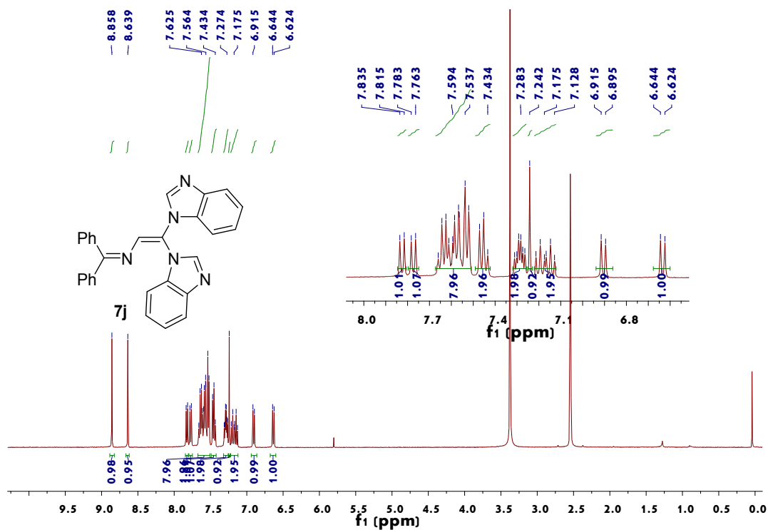
Figure 72. 1 H NMR spectrum of 7j
