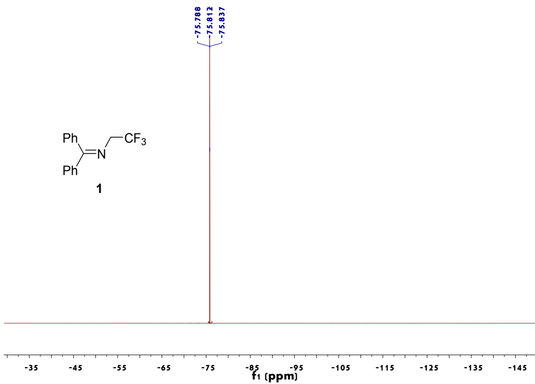
Figure 2. ^{19}\text{F} NMR spectrum of 1
