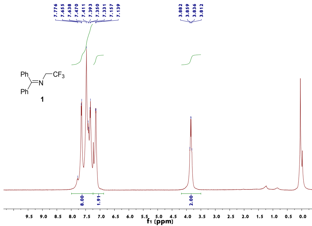
Figure 1. ^1\text{H} NMR spectrum of 1
