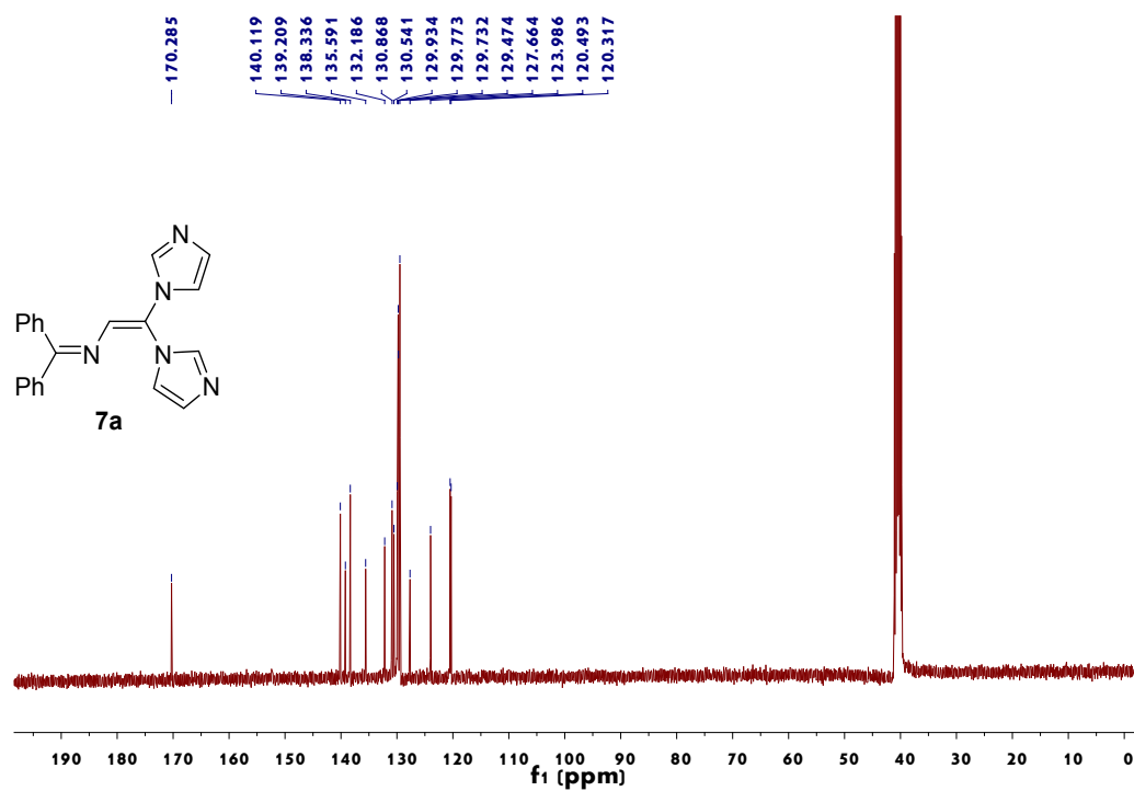
Figure 67. 13 C NMR spectrum of 7a
