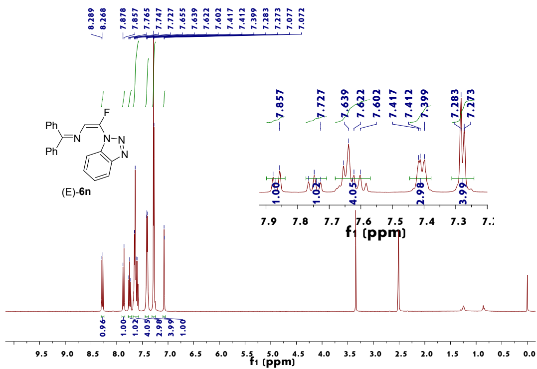
Figure 60. 1 H NMR spectrum of (E)-6n
