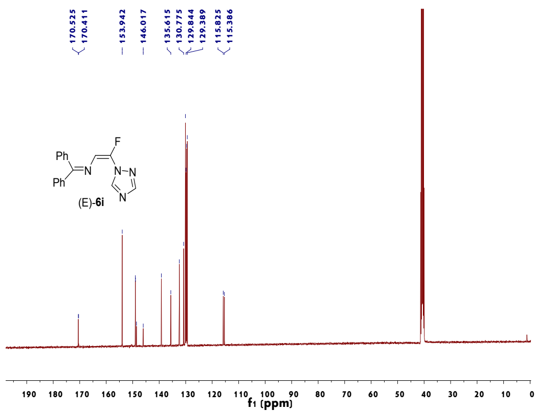
Figure 38. 13 C NMR spectrum of (E)-6i
