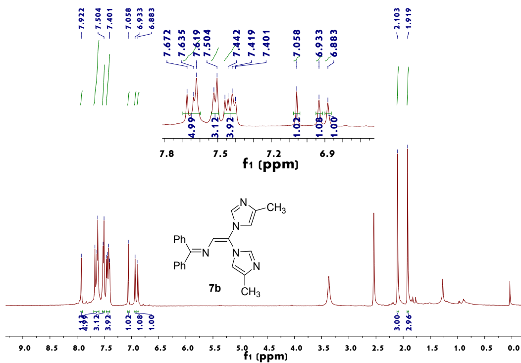
Figure 68. 1 H NMR spectrum of 7b
