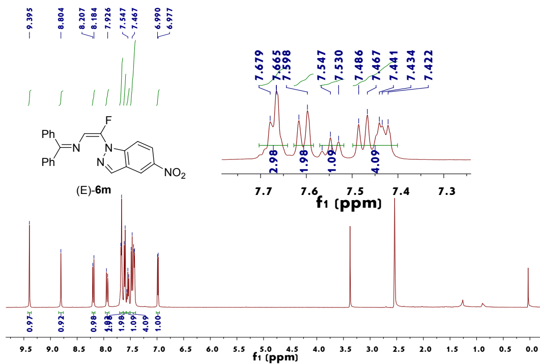
Figure 54. ^1\text{H} NMR spectrum of (E)-6m
