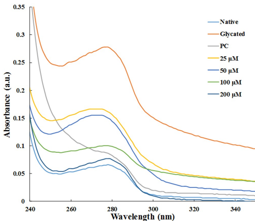
Supplementary Fig. S1. UV-visible spectra of native, glycosylated and treated HSA after 30 days. (PC is aminoguanidine treated). All the data have been expressed in mean \pm SEM for three independent experiments.
