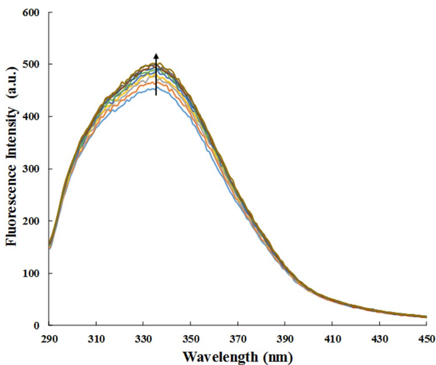
Supplementary Fig. S2. Fluorescence emission spectra of HSA-cinnamic acid complex with varying concentration (0-100 mM) of NaCl.
