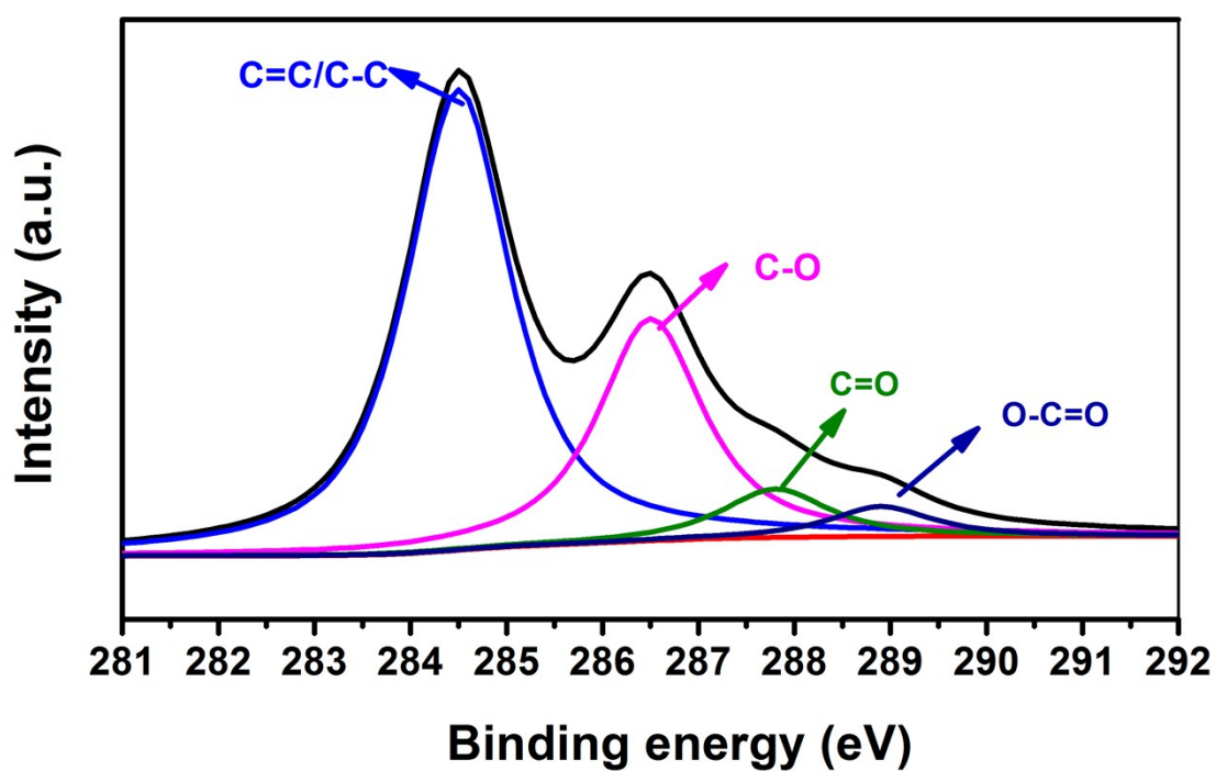
Fig. S2. XPS spectra of GO
