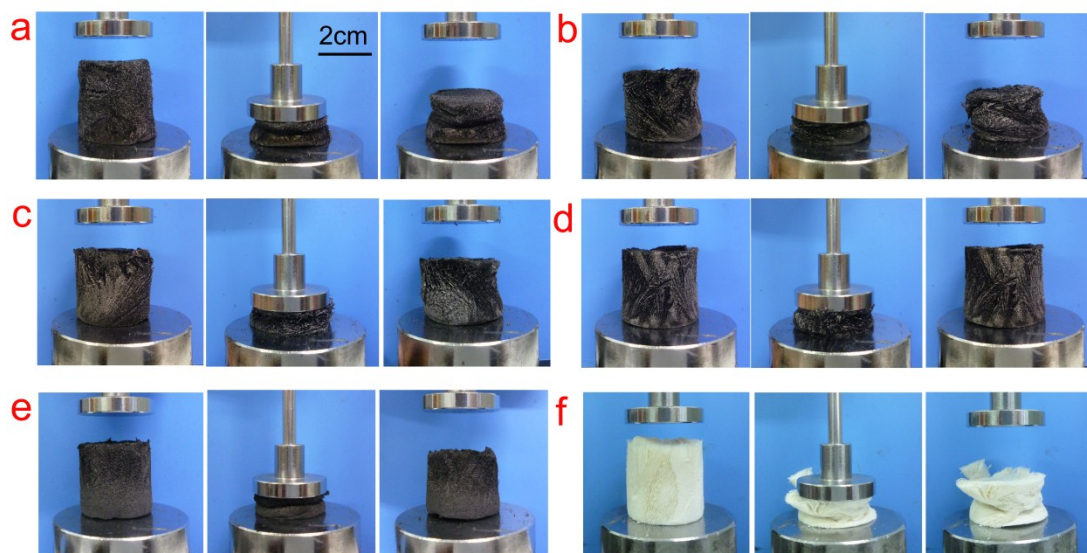
Fig. S3. Photographs showing different aerogels under a compressing and releasing cycle. (a) pure-GO aerogel (b-e) rGO/SA-1, rGO/SA-2, rGO/SA-3 and rGO/SA-4 aerogels (f) pure-SA aerogel.
