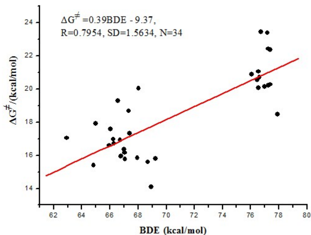
Figure S2. The correlation between \Delta G^\ddagger and BDE.
