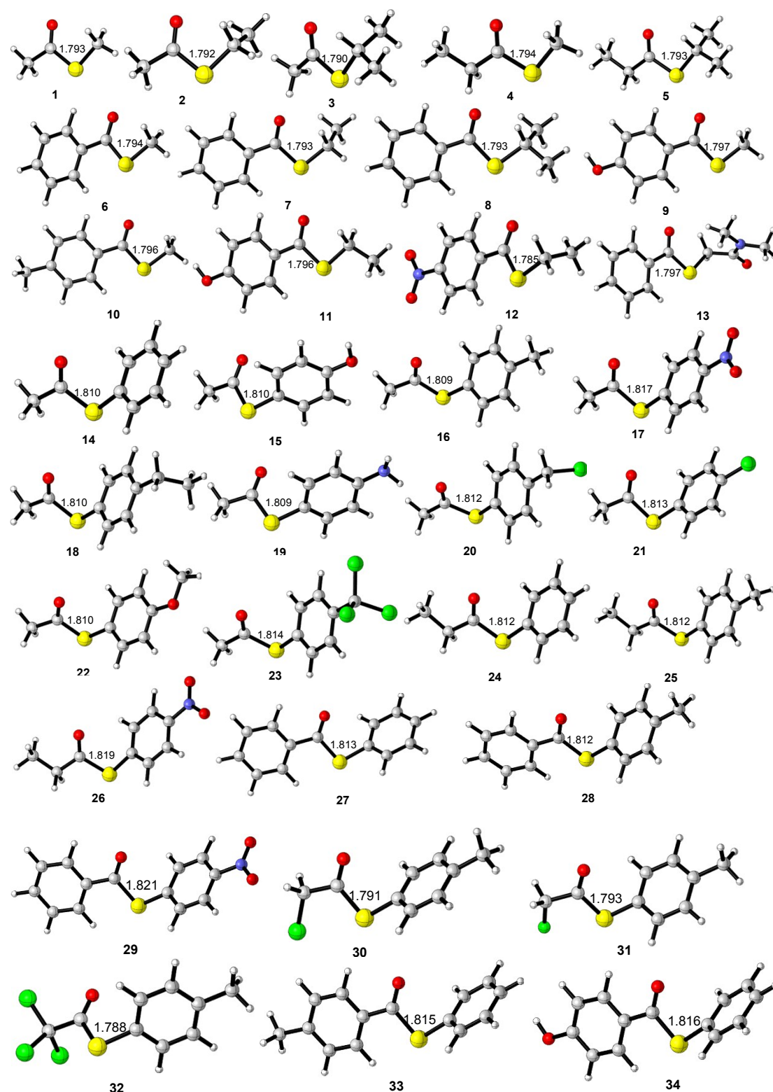
Figure S1. The optimized geometries of 34 thioesters.
