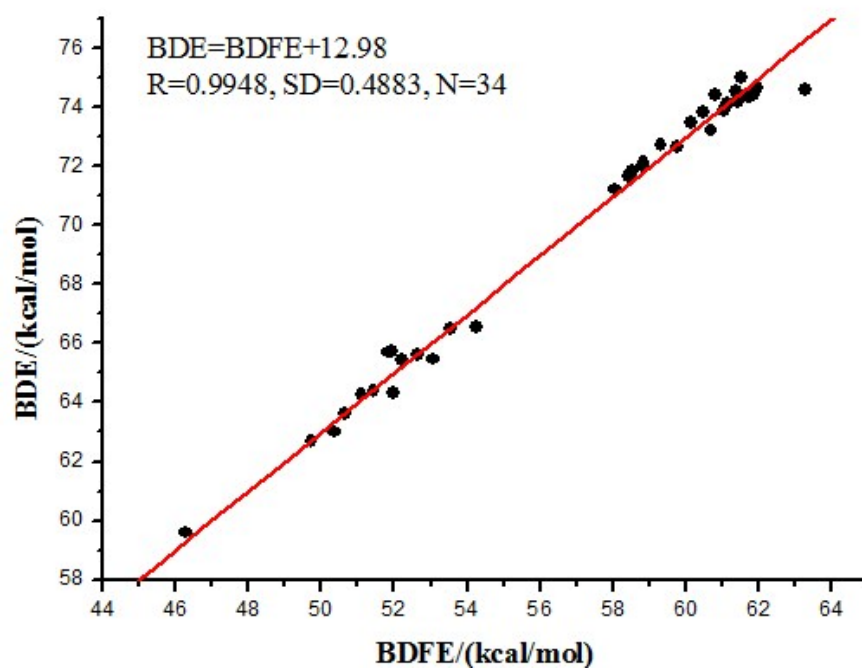
Figure S3. The linear correlation plots between BDE and BDFE values (in solvent).
