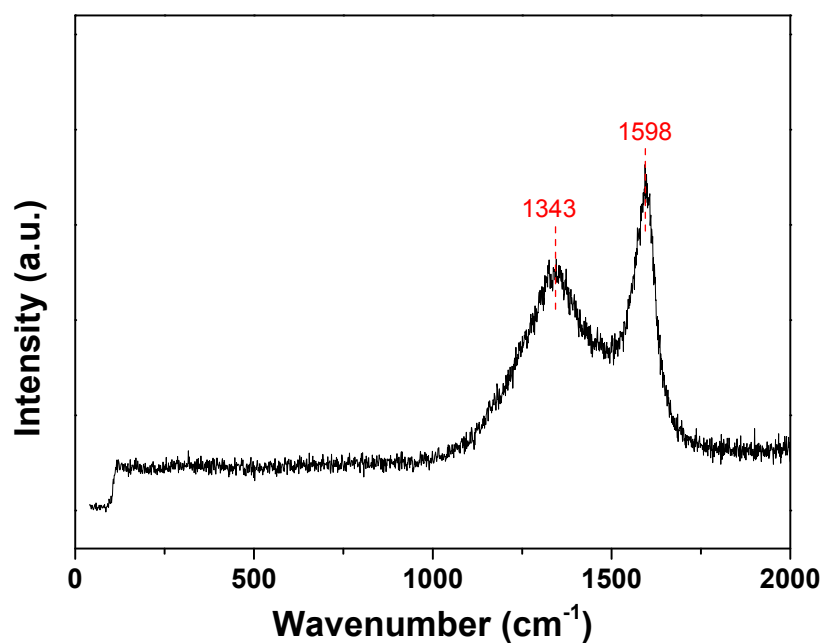
Fig. S1 Raman spectrum of the decomposition product of Fe-BTC
