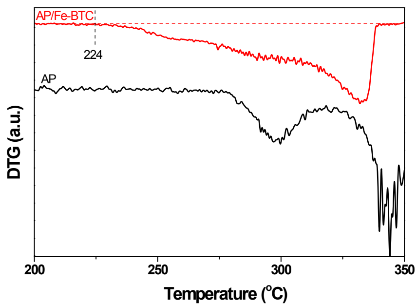
Fig.S2 Enlarged view of the DTG curves of AP with and without Fe-BTC
