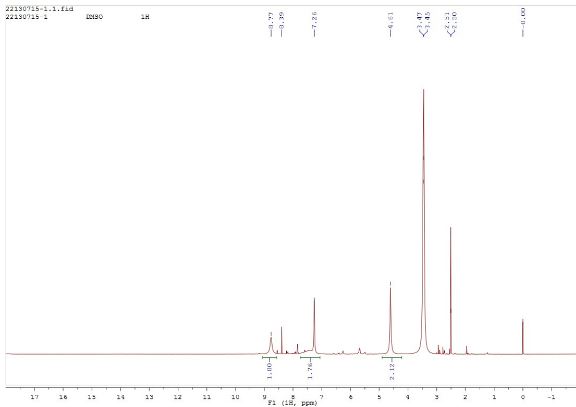
Fig. S1 The ^1\text{H} spectra of the polymer.
