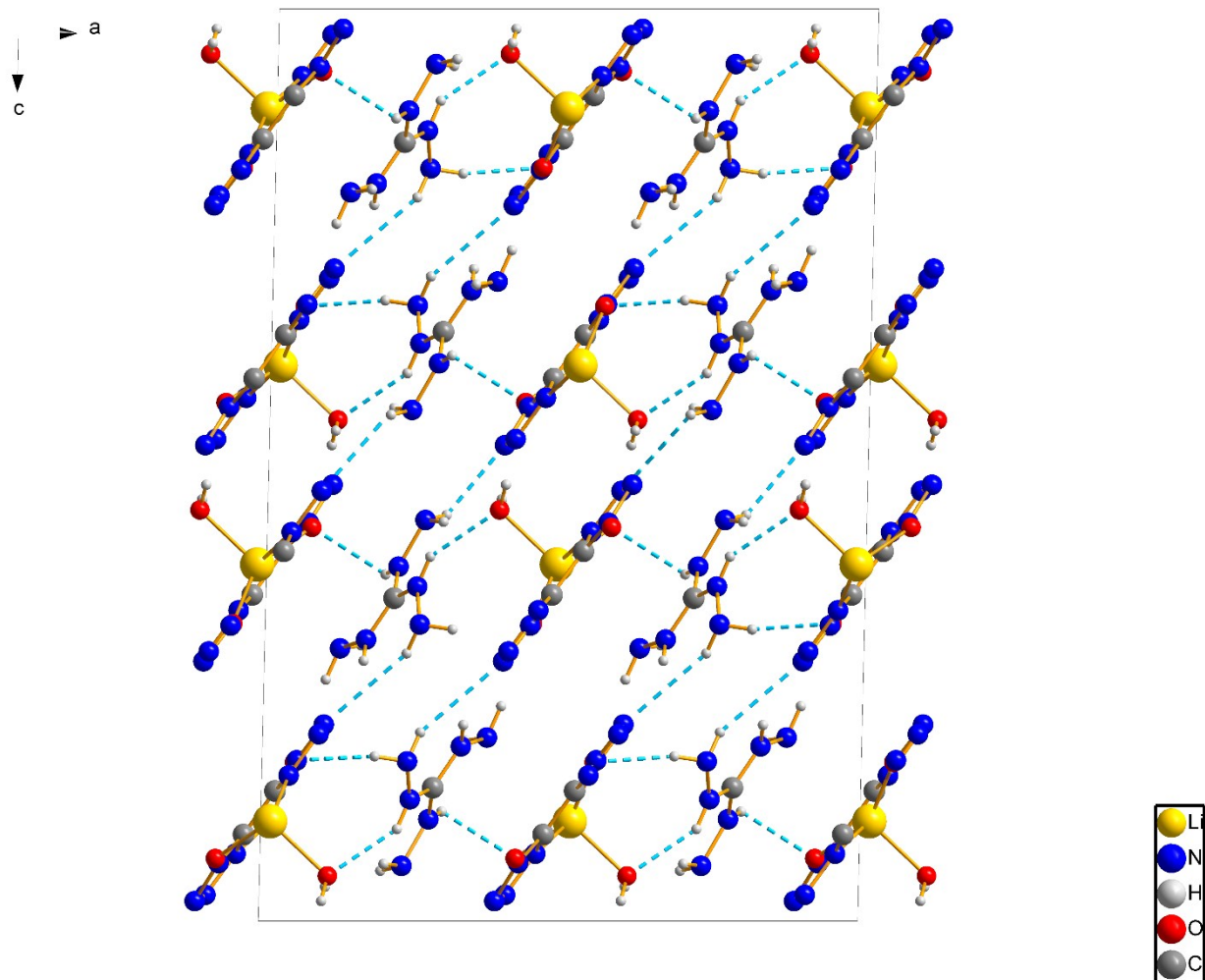
Fig. S6 The packing diagram from b -axis.
