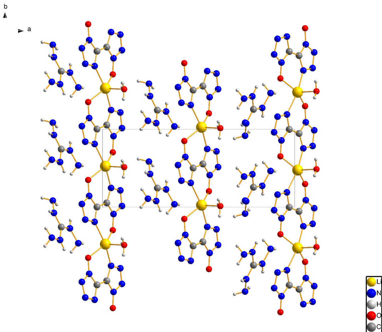
Fig. S7 The packing diagram from c -axis.
