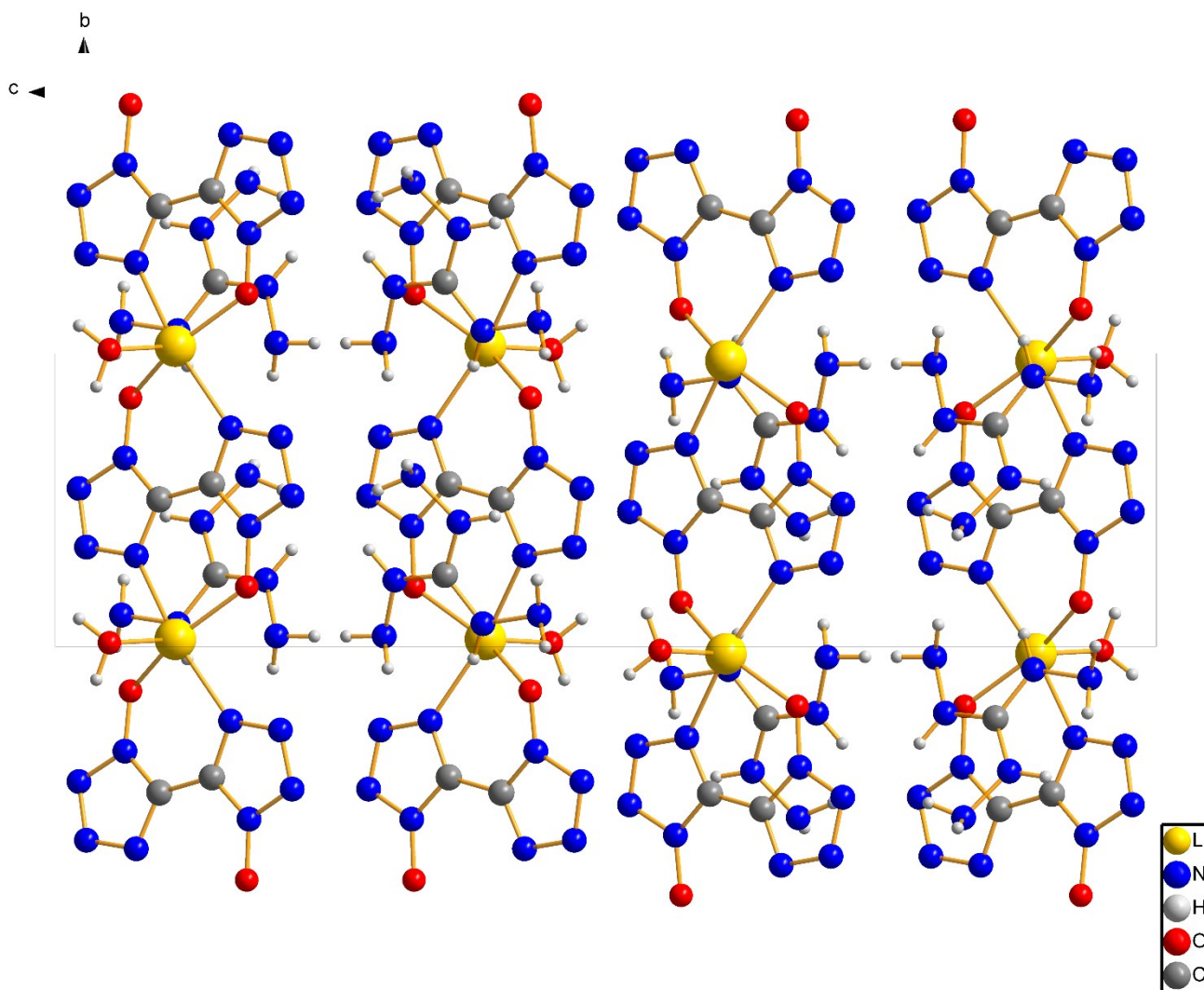
Fig. S5 The packing diagram from a -axis.
