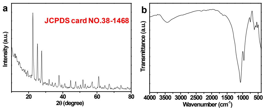
Fig. S1: (a) XRD and (b) FTIR spectra of the 700°C-treated sample (TiP 2 O 7 )
