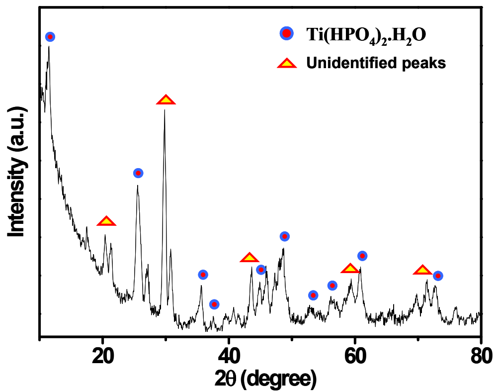
Fig. S5: The XRD plot of the sample after adsorption of Pb(II)
