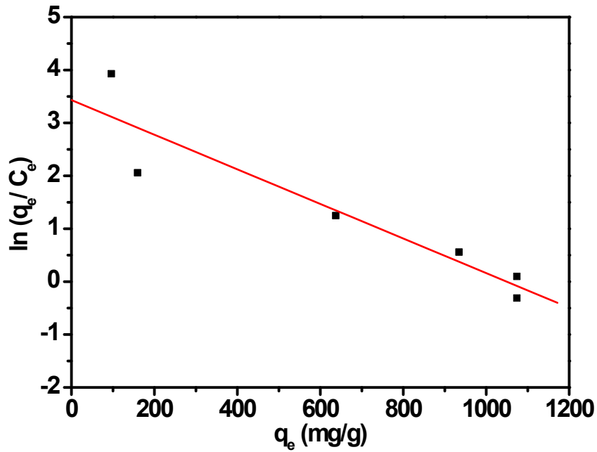
Fig. S4: The plot of \ln(q_e/C_e) Vs. q_e of Pb(II) ion adsorption on the sample
