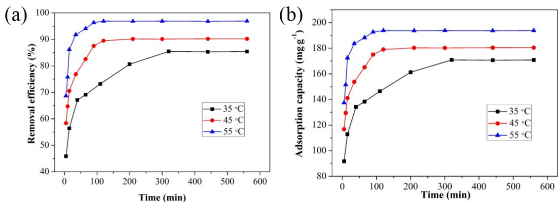
Fig. S1 Effect of temperature on adsorption of Cu (II) by CoFe 2 O 4 @SiO 2 -NH 2 : (a) removal efficiency, and (b) adsorption capacity.
