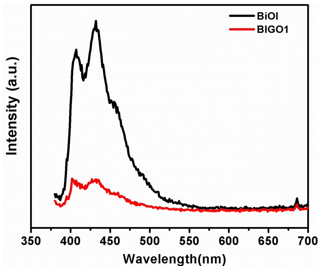
Figure 5 PL spectrum of BiOI (black in color) and BIGO1 nanocomposites (red in color).
