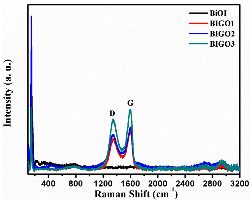
Figure 3 Raman spectrums of as-synthesized samples.
