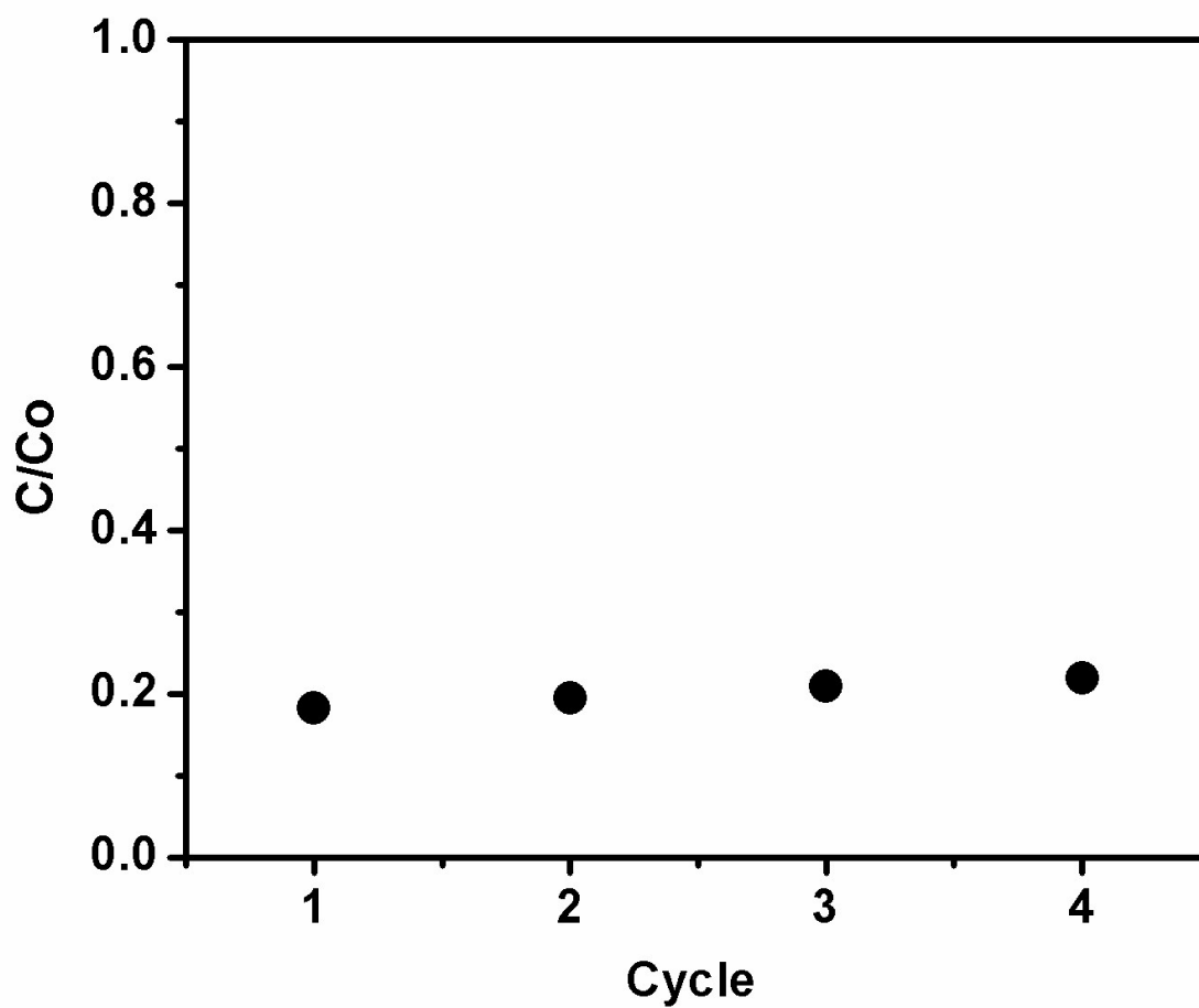
Figure 6 Photocatalytic stability of BIGO1 sample on the degradation of MO under visible light irradiation.
