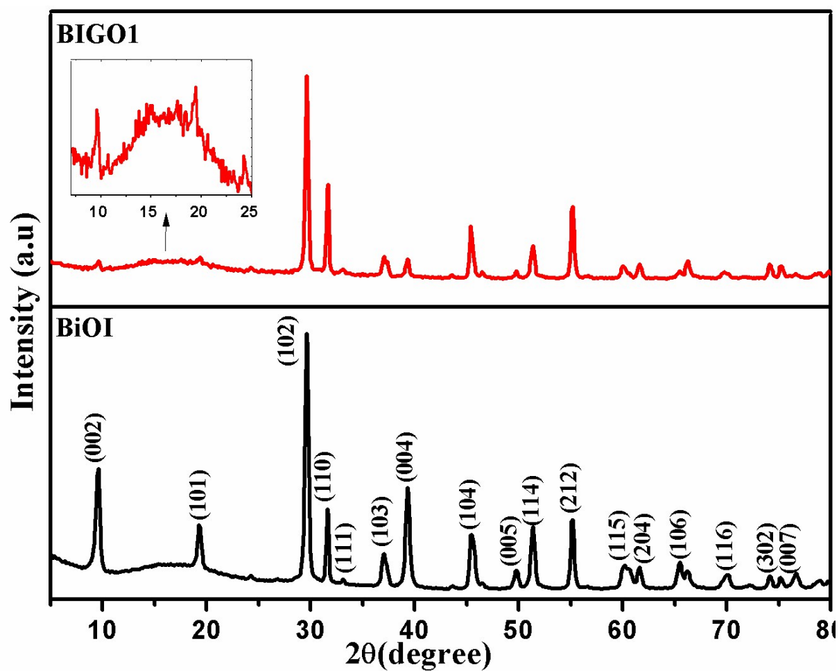
Figure 1 XRD pattern of BiOI (black in colour) and BIGO1 (red in colour).
