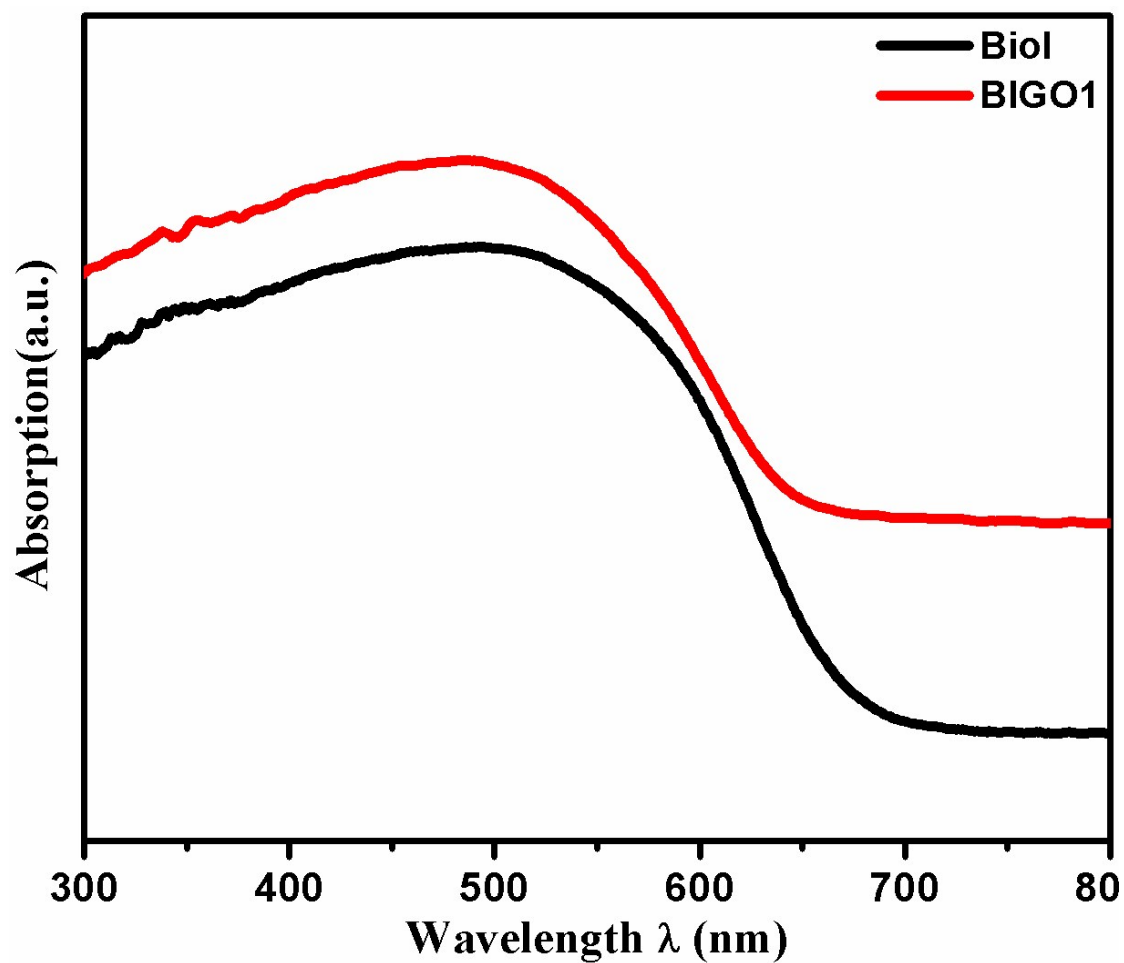
Figure 4 UV-vis spectrum of BiOI (black in color) and BIGO1 nanocomposites (red in color).
