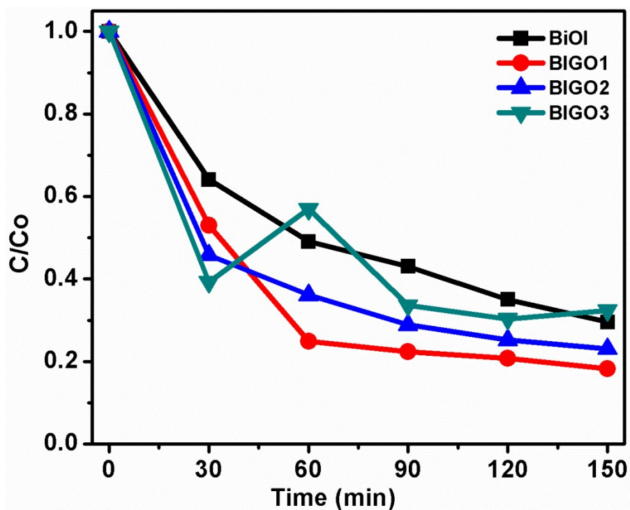
Figure 7 Photocatalytic activities of BiOI and BiOI–GO nanocomposites samples on the degradation of MO under visible light irradiation.
