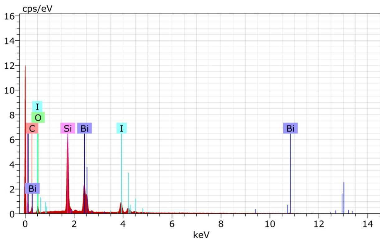
Figure 2 EDS Spectrum of the BIGO1 nanocomposite.
