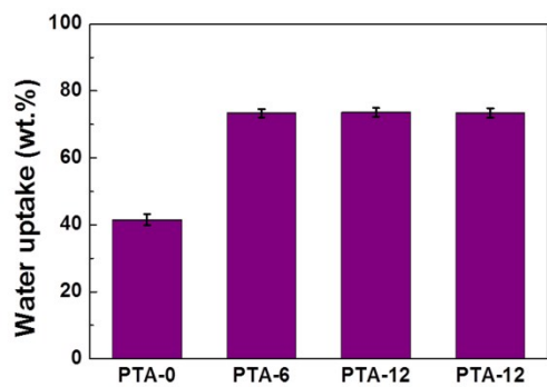
Figure S2. Water uptake content of modified and unmodified PVDF membranes.
