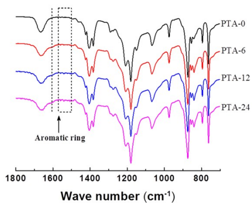
Figure S1. ATR-FTIR spectra of modified and unmodified PVDF membranes.
