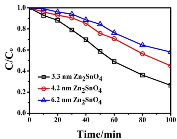
Fig. S2 Photocatalytic activities of Zn_2SnO_4 nanoparticles with different sizes for photodegradation of RhB molecules.
