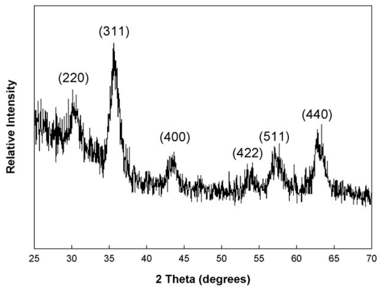
Figure S1: XRD of SPION-OA.
