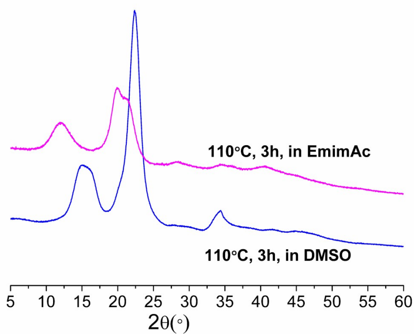
XRD data of pure cellulose pretreated in EmimAc and DMSO at 110°C for 3h.
