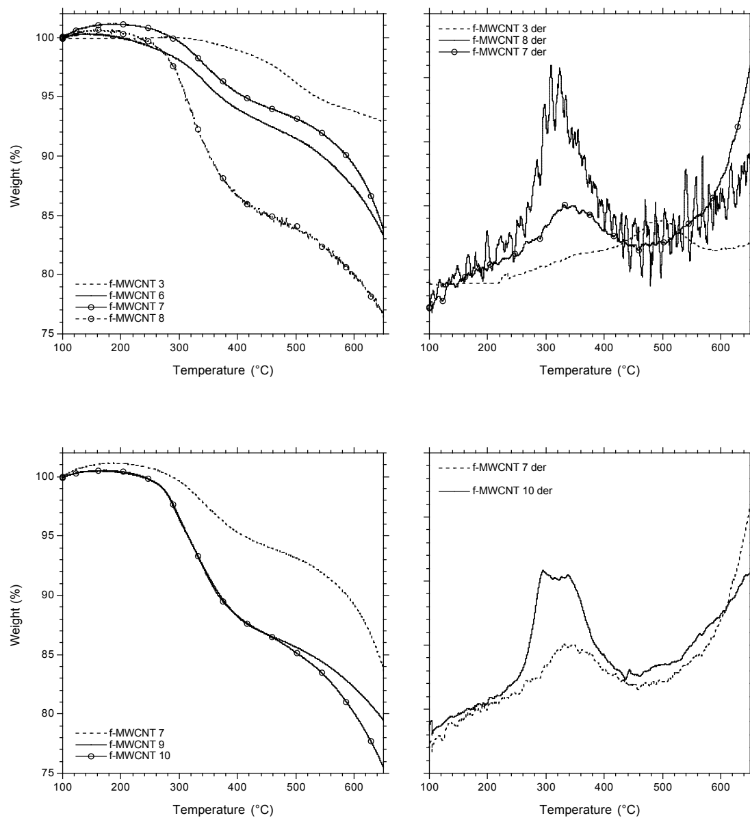
Fig. S1: TGA analyses and derivatives of all compounds.
