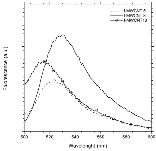
Fig. S2: Fluorescence of f -MWCNT 5, 8, 10 in water.
