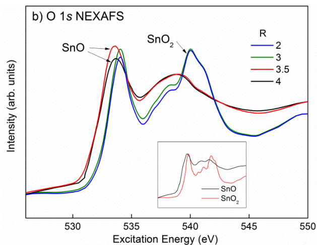
Figure S1. O 1s NEXAFS spectra of Nd-doped SnO x samples versus the Ar/O 2 gas flow ratio. The spectra of SnO and SnO 2 powder shown in the inset of each graph were added for comparison.
