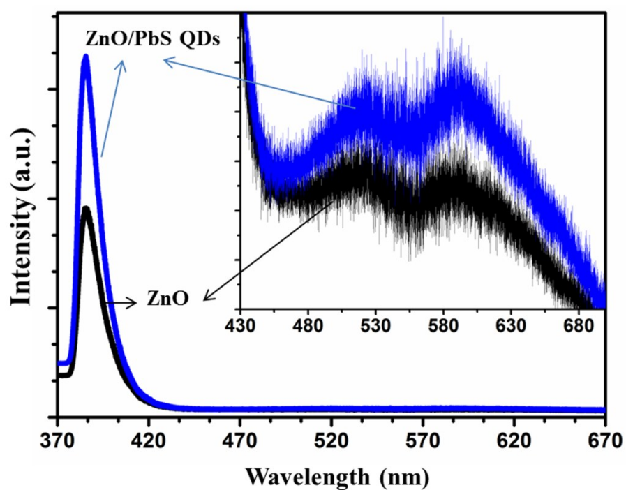
Fig. 1 PL spectrum of ZnO and ZnO/PbS QDs formed by SILAR method with aqueous-containing solution as solvents. Inset is the enlarged spectrum of their visible light emission.
