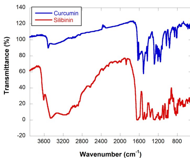
Figure S.1. FTIR spectra of curcumin and silibinin.
