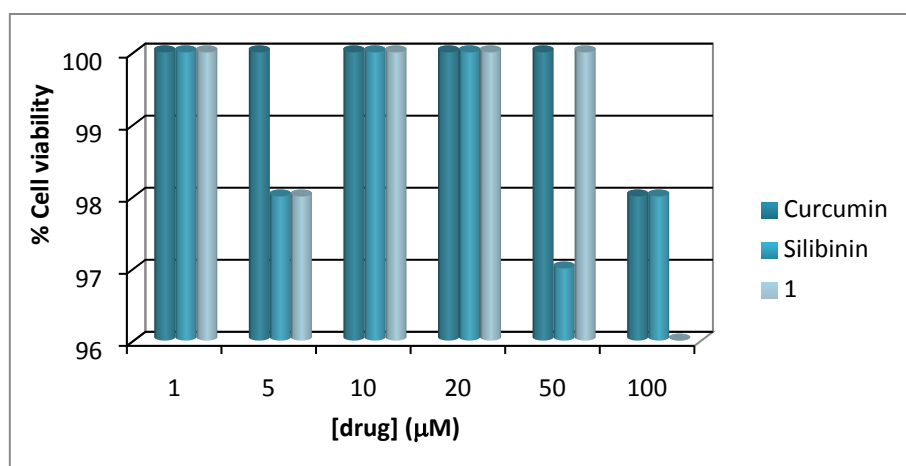
Figure S.3. MTS test for cell viability of 8505c cells cultured for 72 h in presence of 1 , curcumin and silibinin.
