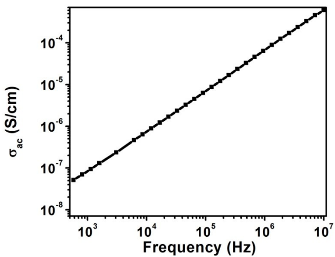
Supplementary Information Figure.1. Frequency dependence of AC electrical conductivity of \text{PbTi}_{0.5}\text{Fe}_{0.5}\text{O}_{3-\delta} nanoparticles at room temperature.
